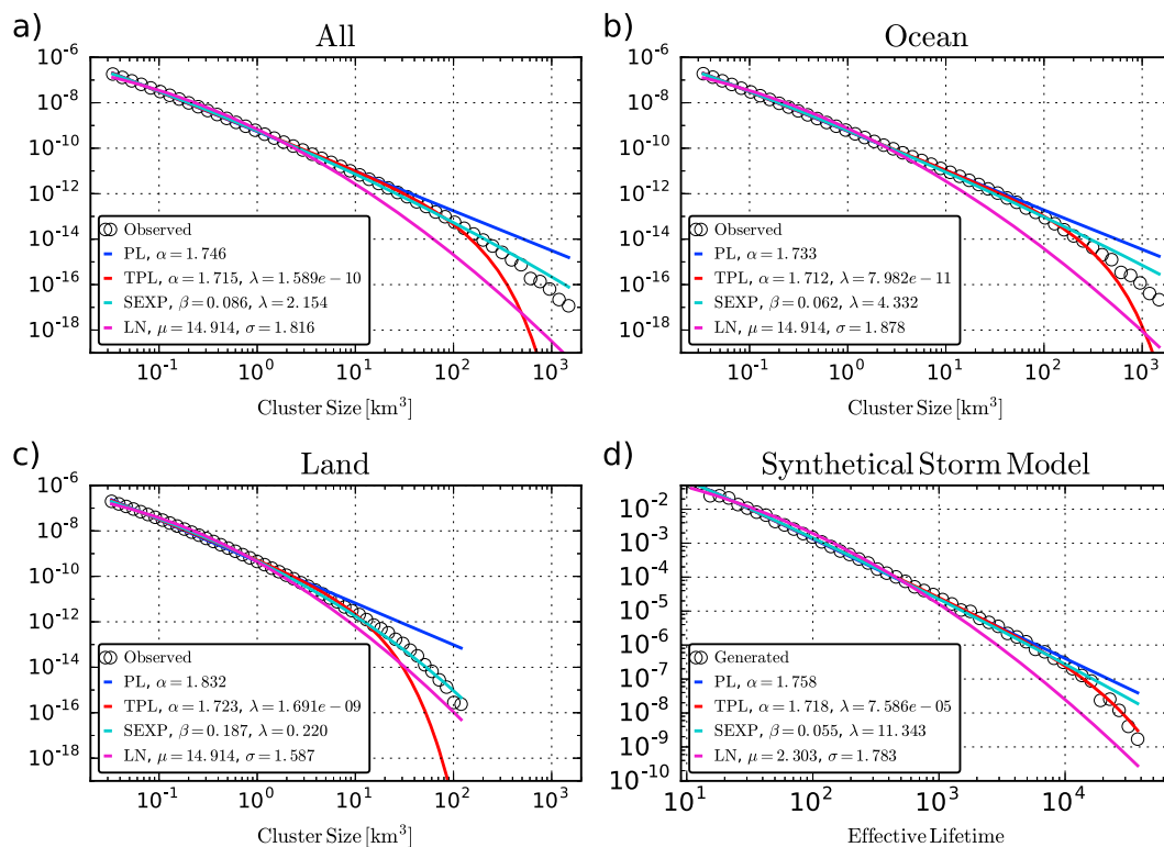
Figure 2. Histograms of the observed spatiotemporal extreme rainfall cluster sizes and the effective lifetimes of the generative model introduced in section 3.3 (circles), as well as the corresponding MLE-optimized fits of the proposed candidate distributions (lines). In all panels, blue lines indicate the optimal power law (PL) fits, red lines the truncated power law (TPL) fits, cyan lines the stretched exponential (SEXP) fits, and magenta lines the lognormal (LN) fits. The respective optimal parameters of the MLE fits are stated in the legends. (a) Histogram of observed cluster sizes for all clusters combined ( n^C \approx 1.42 \cdot 10^7 ) and MLE-fitted cluster size distributions. (b) Histogram of observed cluster sizes for the subset of ocean clusters ( n^C_{\text{ocean}} \approx 8.68 \cdot 10^6 ) and MLE-fitted cluster size distributions for this subset. (c) Histogram of observed cluster sizes for the subset of land clusters ( n^C_{\text{land}} \approx 5.20 \cdot 10^6 ), and MLE-fitted cluster size distributions for this subset. (d) Histogram of effective lifetimes obtained from the generative model introduced in section 3.3 and corresponding MLE-fitted lifetime distributions. Note that the units are arbitrary in this case.
