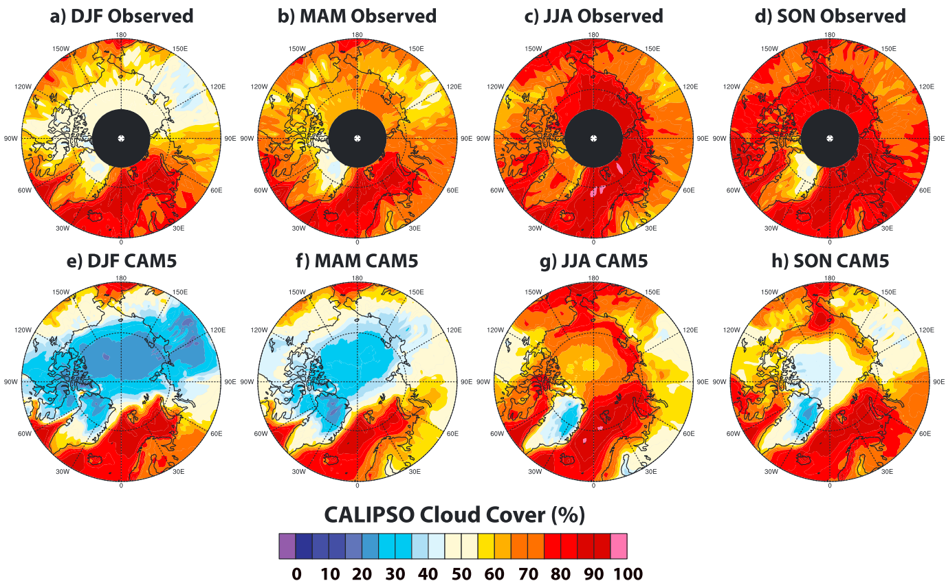
Figure 3. North Pole maps (60–90°N) of total CALIPSO cloud cover (units %) by season: (a) DJF observed, (b) MAM observed, (c) JJA observed, and (d) SON observed. (e–h) Same as in Figures 3a and 3b but for CAM5.
