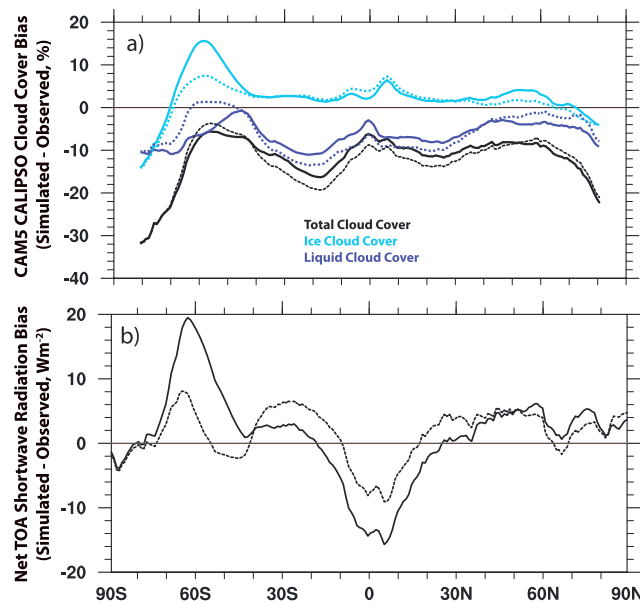
Figure 12. Annual zonal annual mean CAM5 (solid) and CAM5* (dashed) biases (simulated – observed): (a) CALIPSO cloud cover biases (units %) and (b) net top-of-atmosphere (TOA) shortwave radiation bias (units Wm^{-2} ) compared to CERES-EBAF v2.8 [Loeb et al. , 2009]. CAM5* is CAM5 with modifications to shallow convection (see supporting information).
