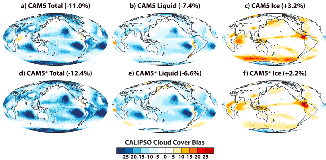
Figure 11. Global maps of CALIPSO cloud cover bias (simulated – observed, units %): (a) CAM5 total, (b) CAM5 liquid, and (c) CAM5 ice. (d–f) Same as in Figures 11a–11c but for CAM5* (CAM5 + modifications to shallow convection; see supporting information).
