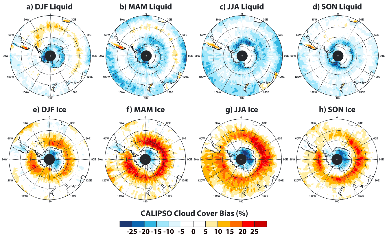
Figure 9. South Pole maps (30–90°S) of CAM5 CALIPSO cloud cover bias (simulated – observed, units %) by season: (a) DJF liquid, (b) MAM liquid, (c) JJA liquid, and (d) SON liquid. (e–h) Same as in Figures 9a–9d but for ice.
