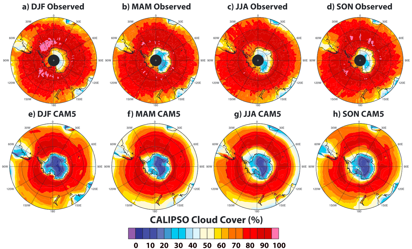
Figure 8. South Pole maps (30–90°S) of total CALIOP cloud cover (units %) by season: (a) observed DJF, (b) observed MAM, (c) observed JJA, and (d) observed SON. (e–h) Same as in Figures 8a–8d but for CAM5.
