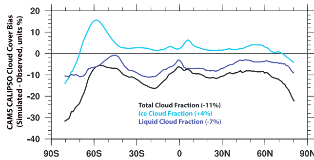
Figure 1. Zonal annual mean CAM5 CALIPSO cloud cover bias (CAM5 simulated – observed, units %). Global mean values are indicated in parenthesis.
