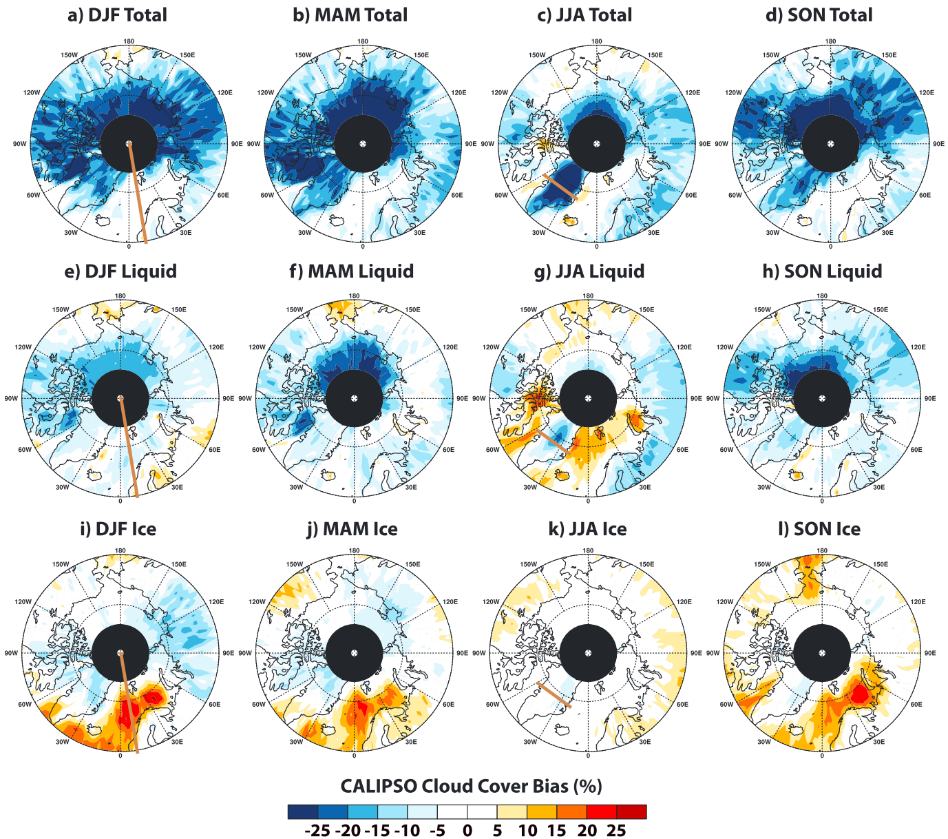
Figure 4. North Pole maps (60–90°N) of CALIPSO cloud cover bias (CAM5 simulated – observed, units %) by season: (a) DJF total, (b) MAM total, (c) JJA total, and (d) SON total. (e–h) Same as in Figures 4a–4d but for liquid cloud cover. (i–l) Same as in Figures 4a–4d but for ice cloud cover. The brown lines indicate the location of the cross section shown in Figures 5a, 5e, and 5i and for Figures 6c, 6g, and 6k.
