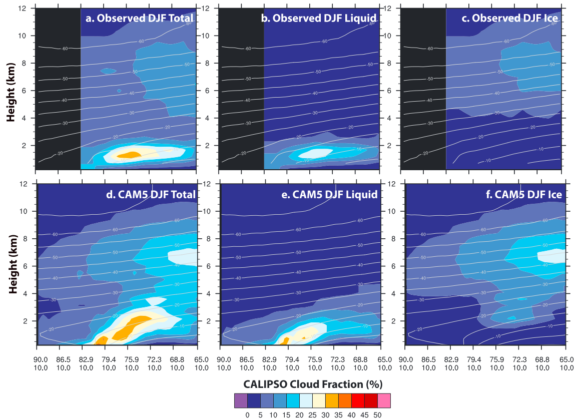
Figure 5. Vertical cross section of CALIPSO clouds and temperatures across the North Atlantic sea ice edge during northern hemisphere winter (DJF): (a) observed total, (b) observed liquid, (c) observed ice, (d) CAM5 simulated total, (e) CAM5 simulated liquid, and (f) CAM5 simulated ice. The contour colors show the CALIPSO cloud fraction (units %), while the grey contour lines show the air temperature (units °C) from ERA-Interim [Dee et al., 2011].
