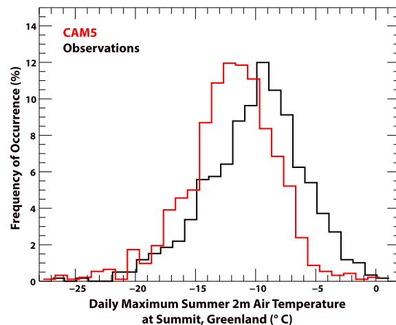
Figure 7. Histogram of daily maximum summer (JJA) 2 m air temperature (units °C) at Summit, Greenland, in CAM5 and observations. Observations from the Global Monitoring Division at the National Oceanic and Atmospheric Administration ( http://www.esrl.noaa.gov/gmd/dv/ftpdata.html ) are shown for the summers from July 2008 to August 2014.
