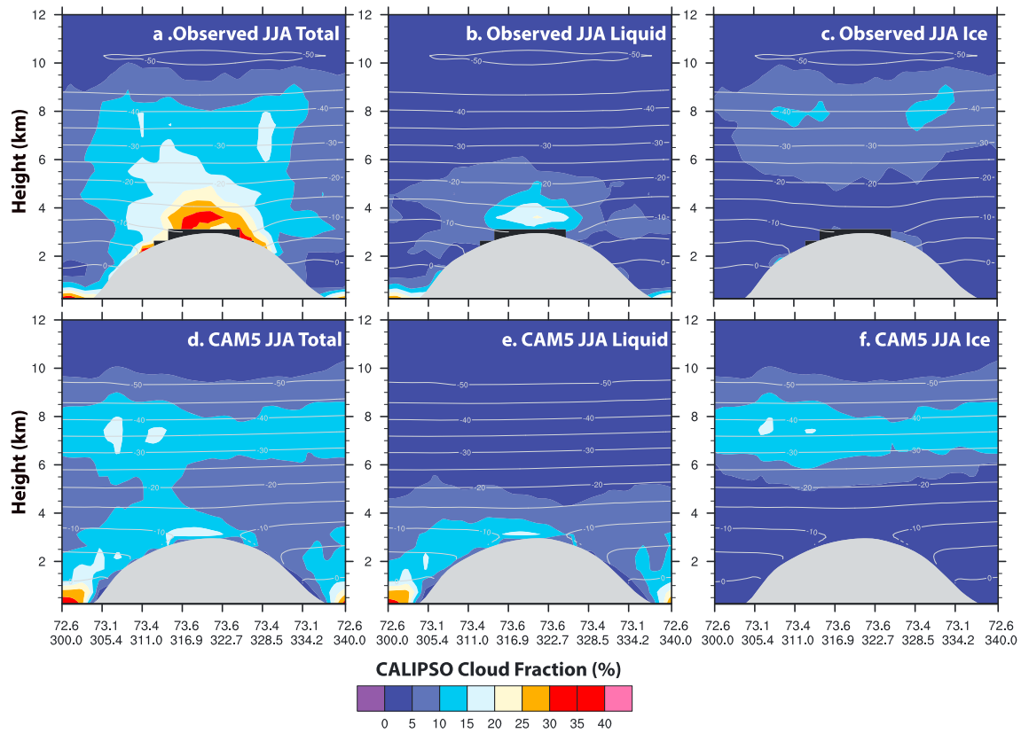
Figure 6. Vertical cross section of CALIPSO clouds and temperatures Greenland during northern hemisphere summer (JJA): (a) observed total, (b) observed liquid, (c) observed ice, (d) CAM5 simulated total, (e) CAM5 simulated liquid, and (f) CAM5 simulated ice. The contour colors show the CALIPSO cloud fraction (units %), while the grey contour lines show the air temperature (units °C) from ERA-Interim [Dee et al., 2011].
