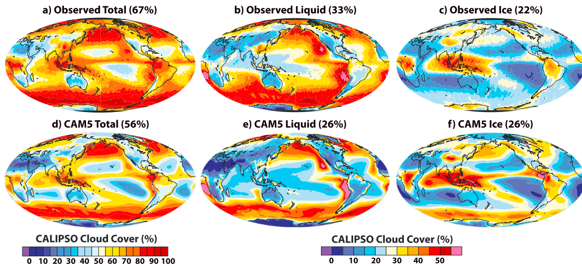
Figure 2. Global maps of CALIPSO cloud cover (units %): (a) observed total, (b) observed liquid, (c) observed ice, (d) CAM5 total, (e) CAM5 liquid, and (f) CAM5 ice. Global mean values are indicated in parenthesis.
