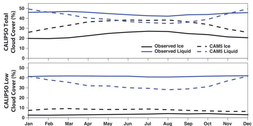
Figure 10. Observed and simulated seasonal cycles of CALIPSO total and low (pressure >680 mb) cloud cover (units %) over the southern hemisphere midlatitude storm track (40–70°S).
