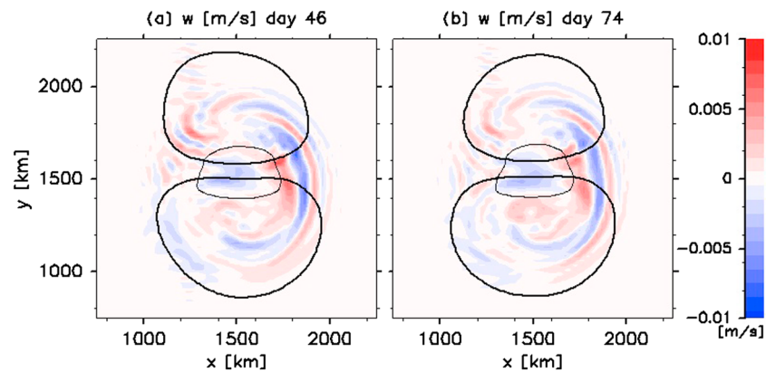
Figure 4. Snapshots of the dipole for Ro = 0.3 in the long-term evolution. Vertical velocity (color shades, m s^{-1} ) at z = 125 m at (a) day 46 and (b) day 74. Dipoles are moved to the center of the domain and rotated by 90° for Figure 4a and 180° for Figure 4b. Black contour lines indicate the positions of the cyclone and anticyclone for each dipole by surface pressure disturbances with \pm 60 Pa. The surface isotach corresponding to |u| = 10 m s^{-1} are also shown by thin contour lines.
