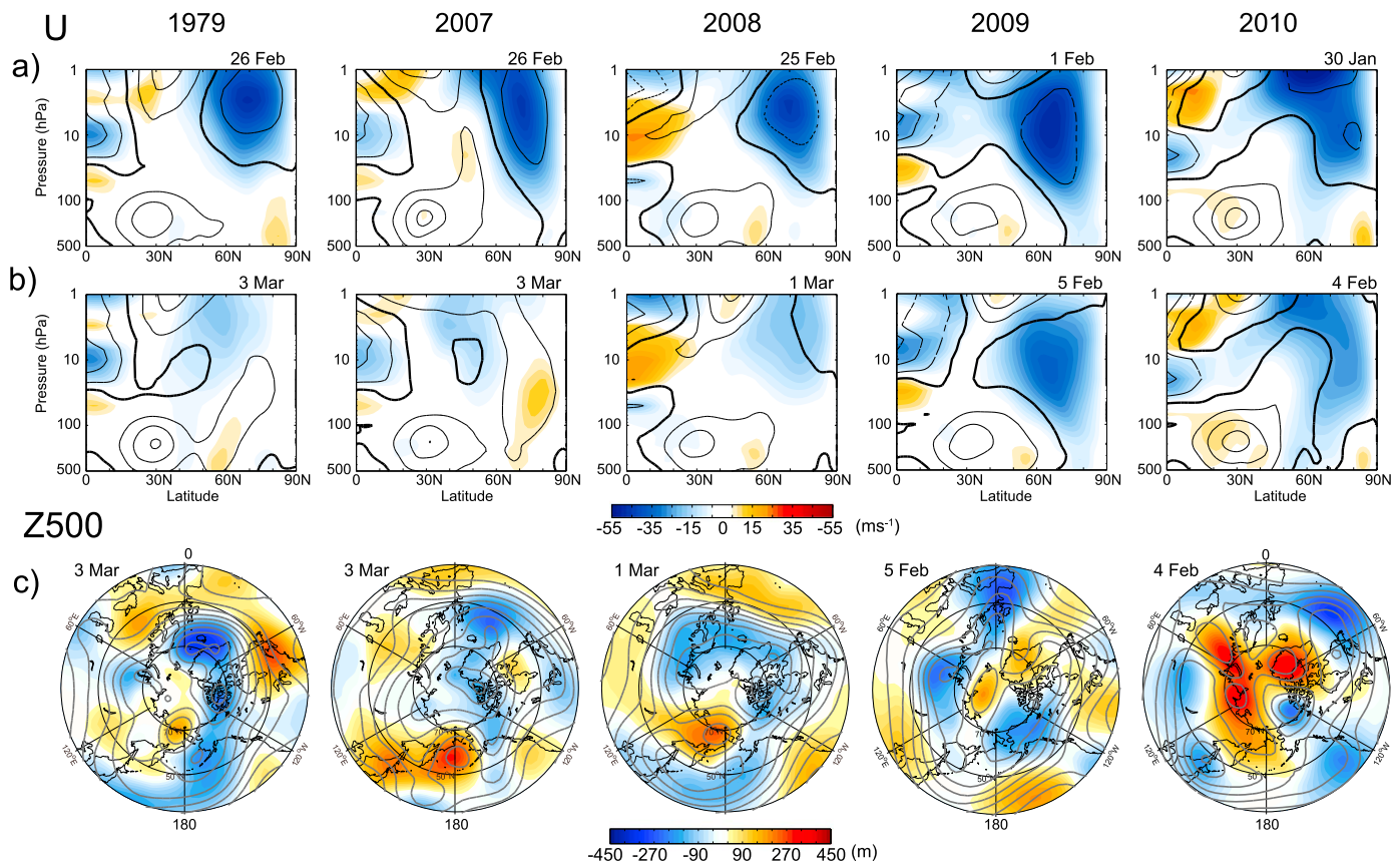
Figure 5. (a) Meridional sections of 5 day mean zonal mean zonal wind (contour interval is 15 m s -1 ; zero contours shown by thick lines) and its anomaly with respect to the climatology (color shading) around T max (vertical lines in Figure 4). The dates indicate central day of the 5 day period. (b) As in Figure 5a, except for 5 days later. (c) 500 hPa geopotential height (contour interval is 100 m) and its anomaly from the climatology (color shading) for dates shown in Figure 5b.
