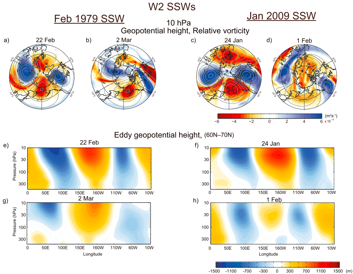
Figure 8. As in Figure 7 except for wave number 2 SSW events for (a, b, e, and g) February 1979 and (c, d, f, and h) January 2009 events. Figures 8a, 8c, 8e, and 8f are around the central date, and Figures 8b, 8d, 8g, and 8h are 8 days later.
