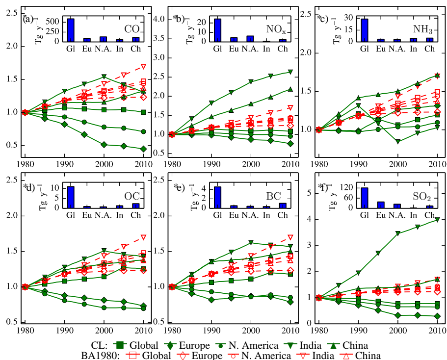
Figure 1. Normalized (to 1980 levels) annual mean anthropogenic emissions of CO, NO x , NH 3 , OC, BC, and SO 2 for the CL (green/solid) and BA1980 (red/dashed) simulations as a function of time. Different regions appear with different symbols: squares for the globe (GL), diamonds for Europe (EU), triangles for China (Ch), inverted triangles for India (In), and circles for North America (N.A.). The histograms at the top of each panel show the absolute emissions in 1980 (used to normalize the emissions) for these regions that are used as reference to normalize emissions (also shown in Table S1).
