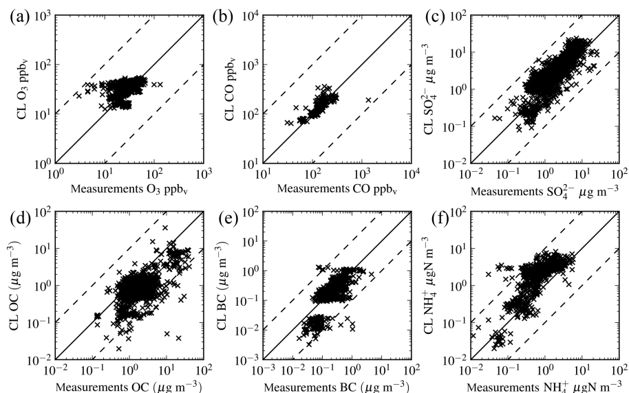
Figure 3. Comparisons of annual average surface model results versus observations per model grid (see Fig. S5 for station locations) for (a) \text{O}_3 , (b) for \text{CO} , (c) \text{SO}_4^{2-} , (d) \text{OC} , (e) \text{BC} , and (f) \text{NH}_4^+ . The continuous line denotes the 1 : 1 slope and the dashed lines the 10 : 1 and 1 : 10 slopes.
