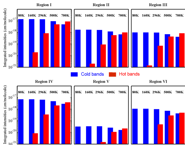
Fig. 16. Integrated intensities (in \text{cm}/\text{molecule} ) for cold- and hot-band transitions from 80 to 700 K in regions I–VI.
