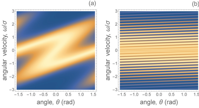
FIG. 1. Filamentation of the phase space density distribution. \Omega/\sigma = 1 , (a) \sigma t = 1 , (b) \sigma t = 15 .
