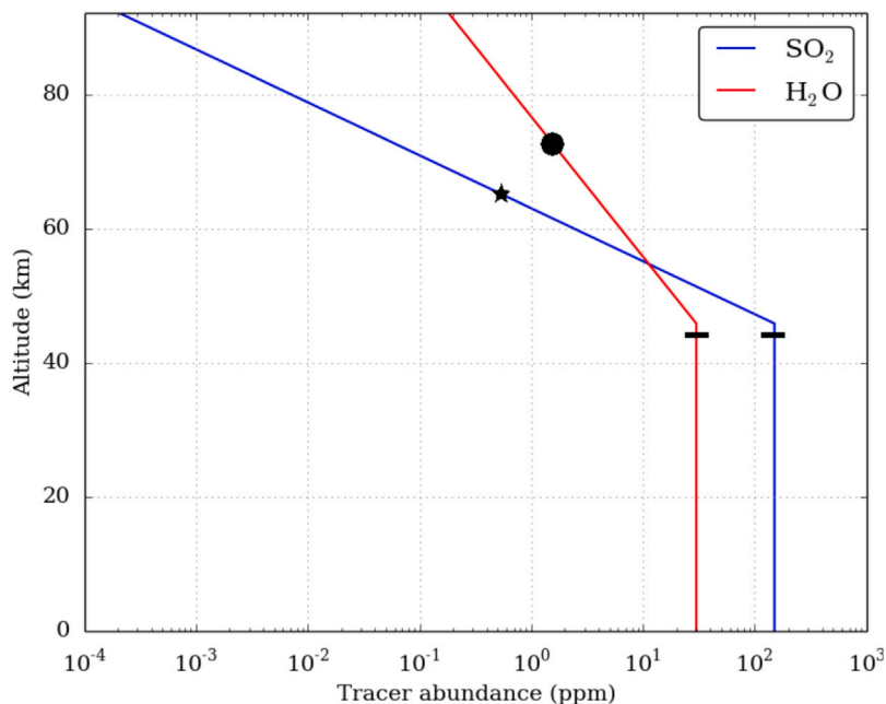
Fig. 1. Vertical relaxation tracer abundance profile (ppm). The circle represents the H 2 O value from Cottini et al. (2012) and Fedorova et al. (2016), the star represents the SO 2 value from Encrenaz et al. (2012, 2015) and the horizontal line represents tropospheric abundance measurements from Bézard and de Bergh (2007).
