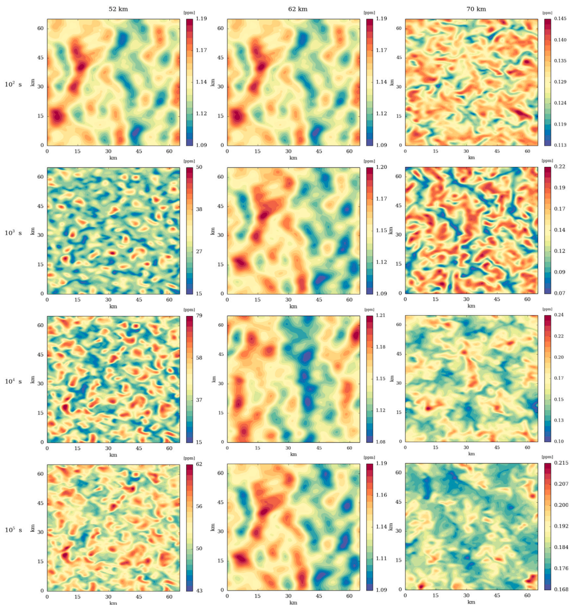
Fig. 4. Instantaneous horizontal cross-section of the tracer abundance (ppm) of SO 2 at the Equator at noon for relaxation timescale values from top to bottom respectively of 10 2 s, 10 3 s, 10 4 s, 10 5 s for 52 km (left column), 62 km (middle column) and 70 km (right column).
