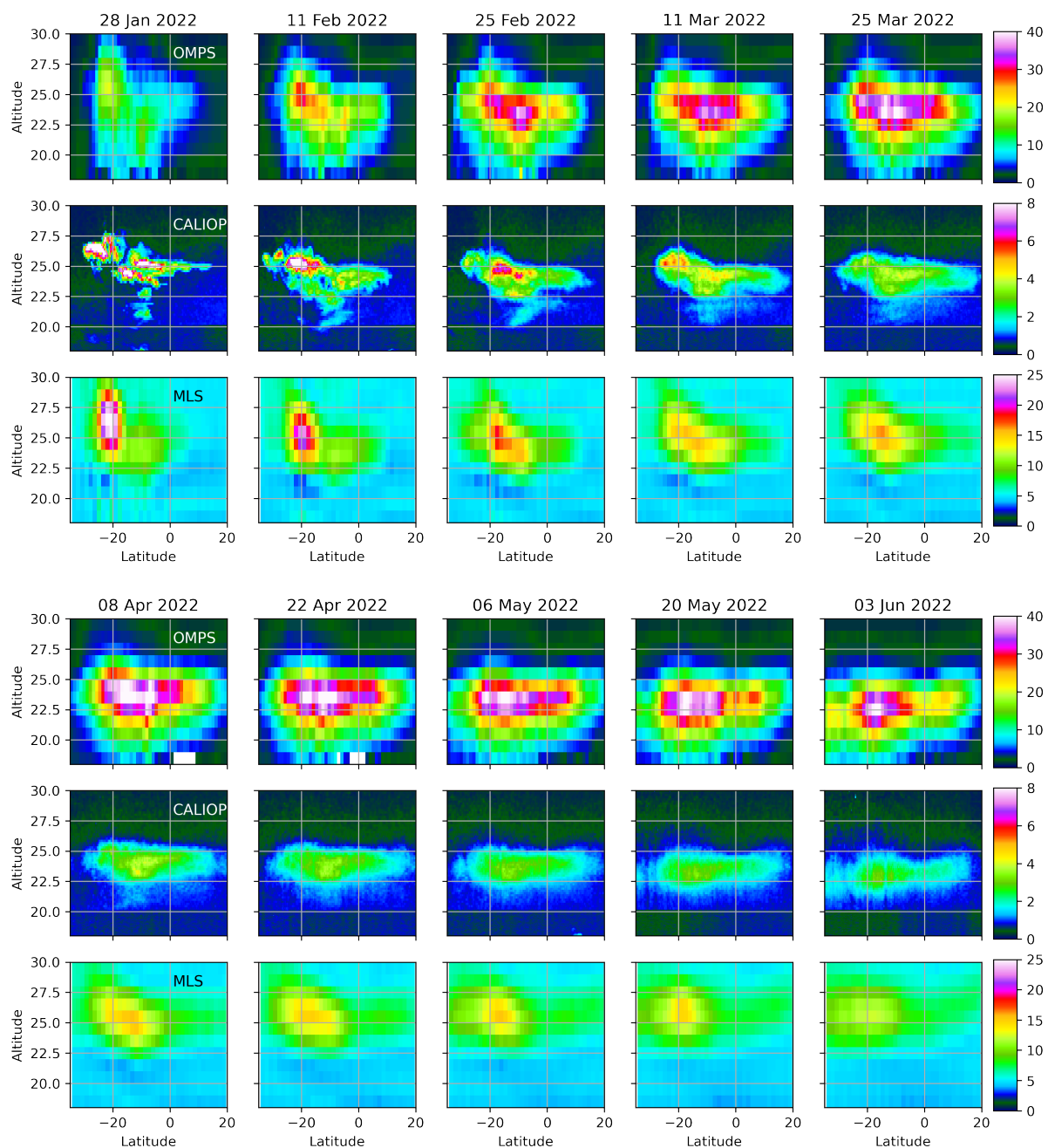
Figure 1. Series of daily zonal averages over all available orbits from three satellites measuring aerosols and water vapour (Appendices A1.3, A1.1 and A1.4). The series is shown in two consecutive blocks of three rows. Upper row: OMPS-LP 745 nm aerosol extinction ratio. Middle row: CALIOP 532 nm aerosol attenuated backscatter ratio. Lower row: MLS water vapour (in ppmv). Days from 28/01/2022 to 04/06/2022 with 16-day step.
