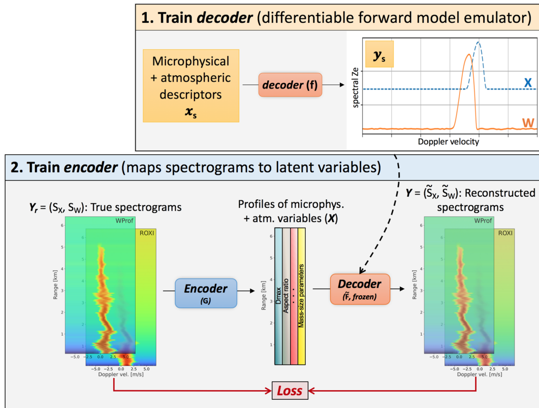
Figure 1. Schematic illustration of the method. The notations are those of Sect. 2.2. The upper right box illustrates that the decoder neural network (NN) is trained to emulate a forward radiative transfer model. The lower box shows the full pipeline where the pretrained decoder is used to reconstruct full spectrograms based on the microphysical properties output by the encoder NN.
