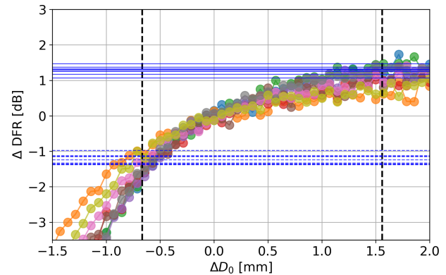
Figure 14. Colored lines with scattered points: \Delta\text{SDFR} caused by adding a diameter offset \Delta D_0 on microphysical descriptors of selected (time, range) gates. Horizontal lines: for each of these (time, range) gates, maximum \Delta\text{DFR} (positive and negative) caused by a modification of the SSRGA coefficients within \pm 10\% . For each selected (time, range) gate, the intersection of the horizontal and colored lines gives a \Delta D_0 value which causes the same change in DFR as a change in SSRGA coefficients (worst case). Dashed vertical lines show the mean of these \Delta D_0 values.
