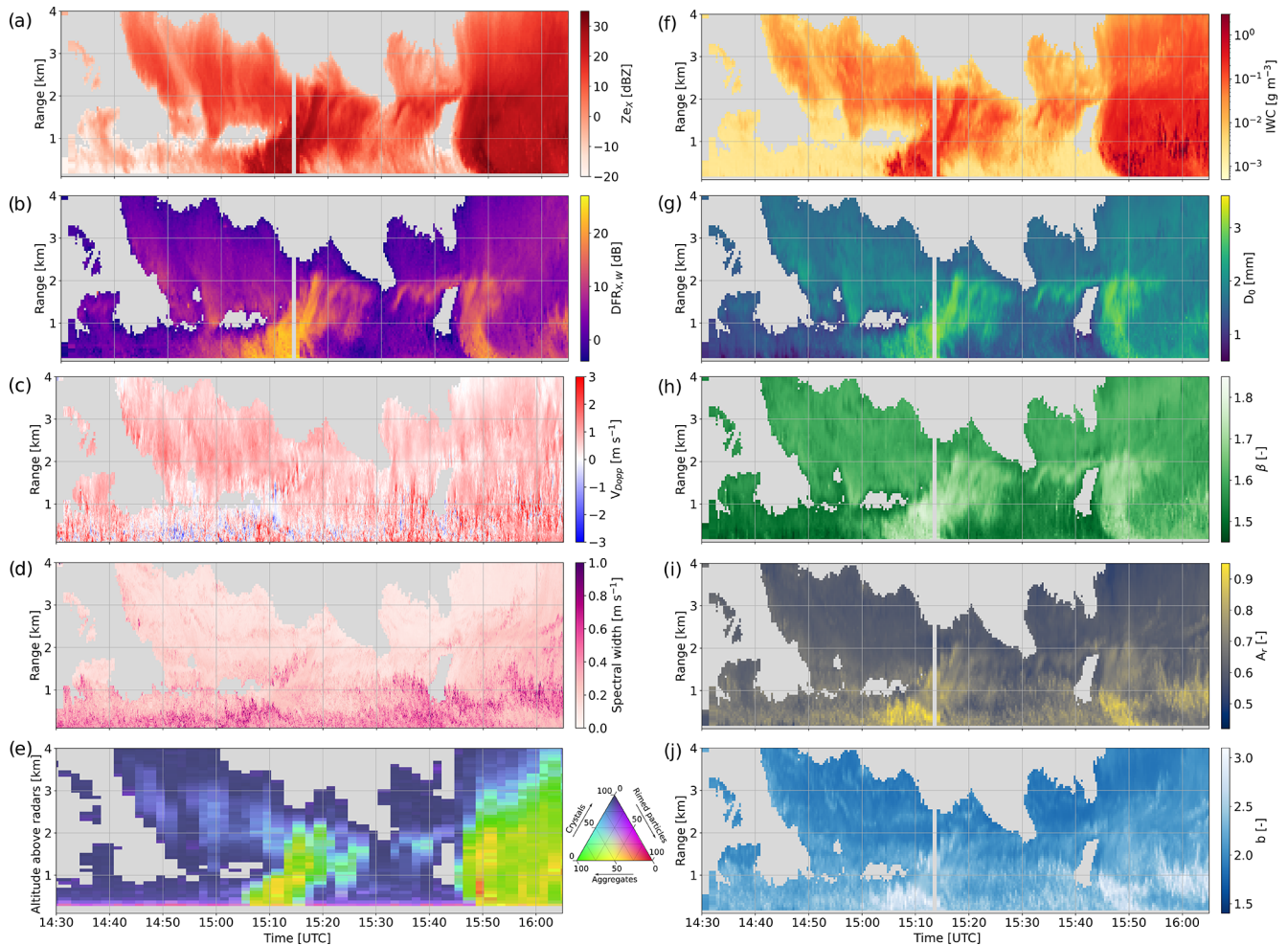
Figure 5. Height–time plots of radar measurements and microphysical retrievals. The left panels contain radar data: (a) Z_{ex} ; (b) DFR_{X,W} ; (c) W-band mean Doppler velocity; (d) W-band spectral width; and (e) time series of hydrometeor classification with demixing showing the proportion of the three main particle types identified – here, aggregates, rimed particles, and crystals (see Sect. 3.3). The right panels feature microphysical retrievals: (f) ice water content, (g) size parameter D_0 , (h) area–size exponent \beta_a , (i) aspect ratio A_r , and (j) mass–size exponent b_m .
