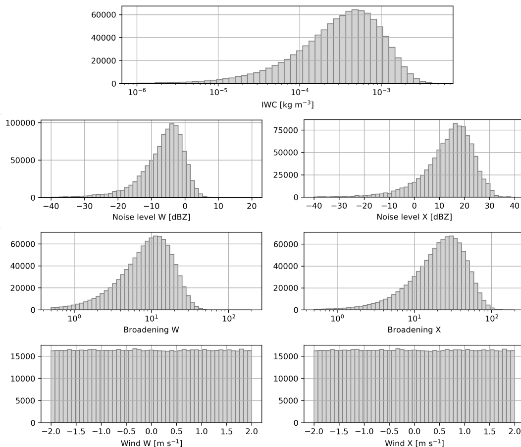
Figure B2. Same as B1 but for the other microphysical descriptors, not provided in MASCDDB.
