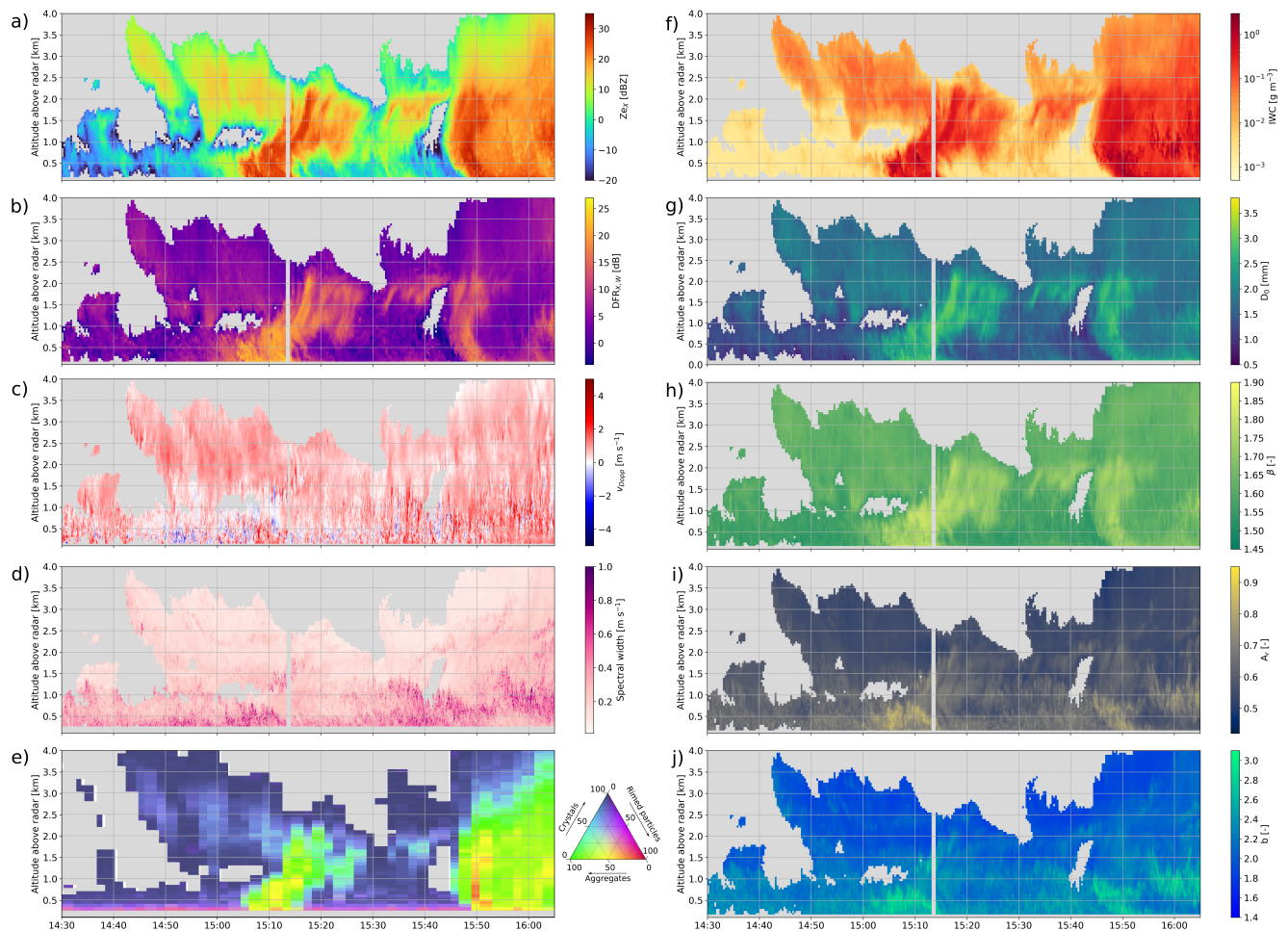
Figure 5. Height-time plots of radar measurements and microphysical retrievals. The left panels contain radar data: a) Z_{eX} , b) DFR_w , c) W-band mean Doppler velocity, d) W-band spectral width, e) Timeseries of hydrometeor classification with demixing showing the proportion of the three main particle types identified: here aggregates, rimed particles and crystals (cf. Section 3.3). The right panels feature microphysical retrievals: f) ice water content, g) size parameter D_0 , h) area-size exponent \beta_a , i) aspect ratio A_r , j) mass-size exponent b .
