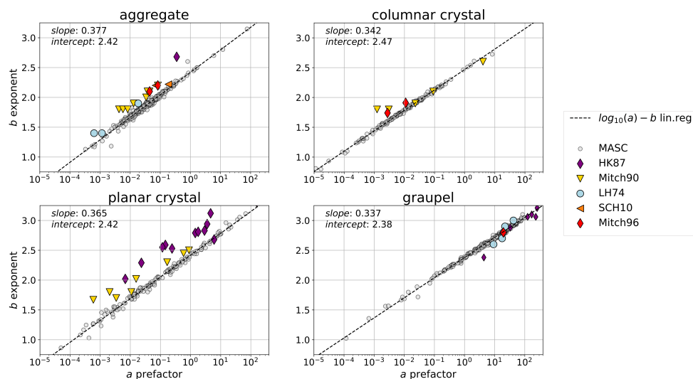
Figure B3. Relation between exponent and prefactor of mass-size relations for different particle types, computed using MASCSDB.
