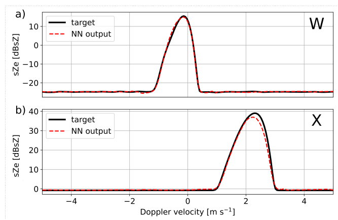
Figure 3. Examples of testing set results for W- and X-band retrievals, with model output (dashed red) and target spectrum (black line). The examples were chosen to reflect some of the typical behaviors and possible artifacts that were observed. Units of spectral reflectivity are used, i.e. 1 \text{ dBsZ} = 10 \log_{10}(1 \text{ mm}^6 \text{ m}^{-3} (\text{ms}^{-1})^{-1}) . Doppler velocity is positive for downward motion.
