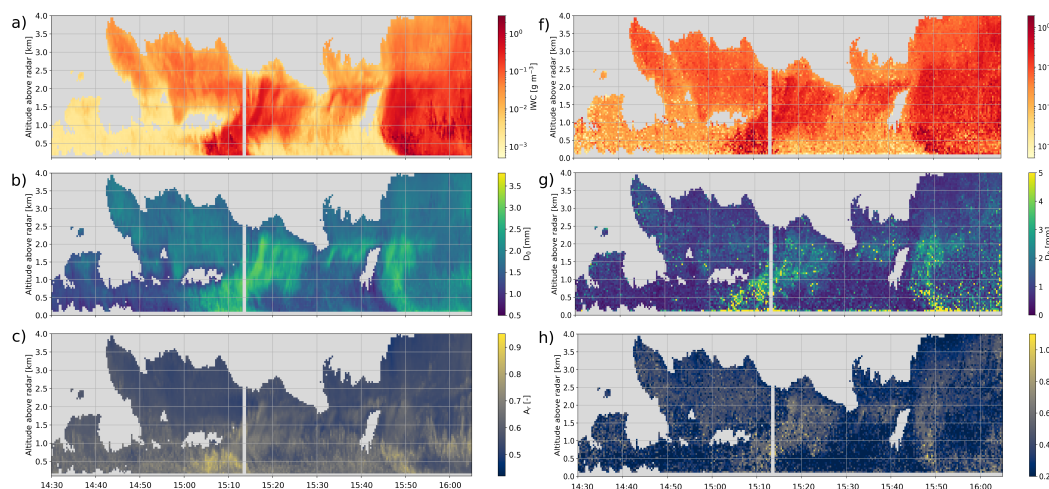
Figure C1. Comparison of timeseries for three examples of variables ( IWC , D_0 and A_r ) retrieved through the proposed framework (left panels) or a direct deep-learning retrieval (right panels). Note that the colorbars may differ (adjusted to reflect at best the variability in each field).
