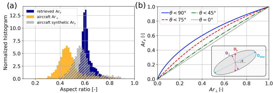
Figure 11. (a) Histogram of retrieved and aircraft-measured aspect ratio. (b) Illustration of the relation between A_{r,\perp} and A_{r,v} for particles with random orientation within a given angle \theta ; the various quantities are sketched in the bottom right of panel (b).
