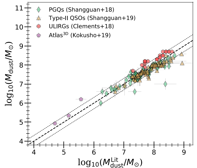
Figure 2. Comparison between our dust masses inferred from the 100/160 \mu\text{m} flux ratios (ordinate), and M_{\text{dust}}^{\text{Lit}} , found in the literature, for the PGQs (Shangguan et al. 2018), Type-II QSOs (Shangguan & Ho 2019), ULIRGs (Clements et al. 2018), and the Atlas 3D (Kokusho et al. 2019) samples (see keys). In each case \beta_{\text{cold}} was chosen to best match the adopted method of the corresponding archival studies (see text). The thick and the thin dashed lines show unity and a factor of 2 deviation from the latter, respectively.
