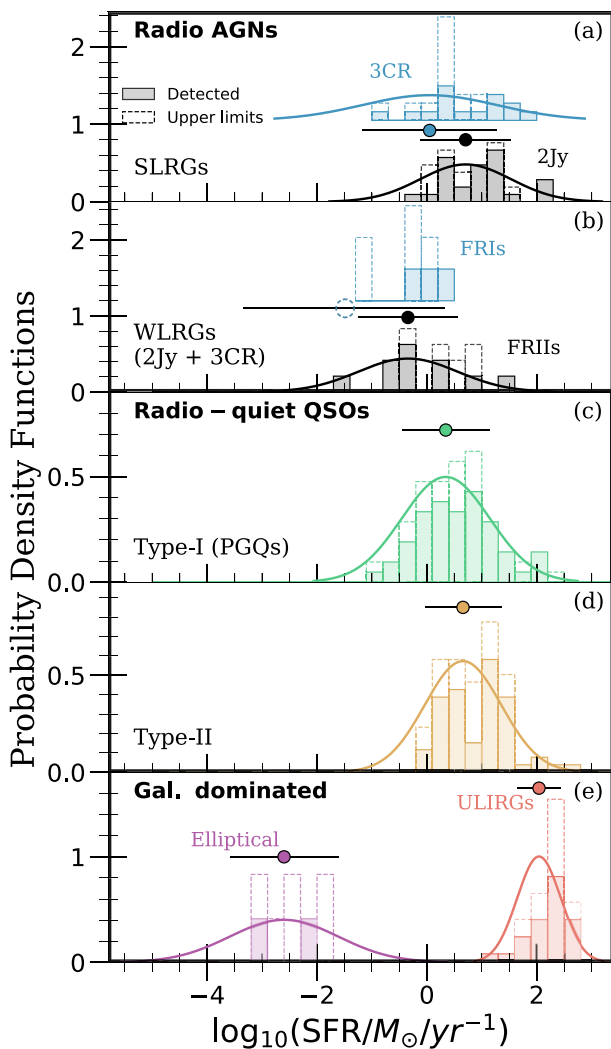
Figure 5. Same as Fig. 4, but for the SFRs.
