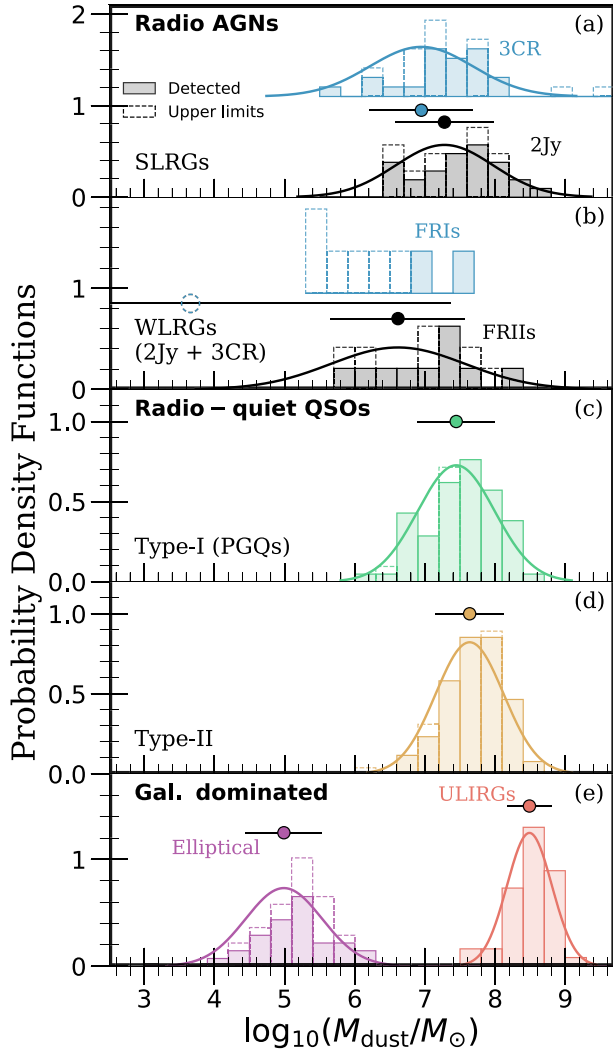
Figure 4. The distributions of M_{\text{dust}} for each of our populations and subsamples of galaxies. Panels (a) and (b) are for radio AGNs, split in terms of SLRGs – panel (a) – and WLRGs – panel (b). We further subdivided the SLRGs into the 2Jy and 3CR samples, and the WLRGs (combining the 2Jy and 3CR samples) into FRIs and FRIIs [these further subdivisions are shown by offsetting one of the histograms in panels (a) and (b)]. Panels (c) and (d) are for radio-quiet QSOs split in terms of Type-I – panel (c) – and Type-II – panel (d) – AGNs. Panel (e) shows the galaxy-dominated samples, including the non-AGN classical elliptical galaxies (purple histogram), and the ULIRGs (orange histogram). The histograms show the observed PDFs of M_{\text{dust}} , where filled bars correspond to the contribution from detected sources, and empty dashed bars from any additional upper limits. The smooth lognormal distributions show the best model PDFs, which account for upper limits. The best-fitting parameters are shown with colour-filled circles (medians \mu ) and error bars (uncertainties \sigma_d ) above or below each of their corresponding PDFs. For WLRG/FRIIs we do not show the fitted PDF, and we show the average parameters with an open dashed circle since they are mostly constrained by upper limits.
