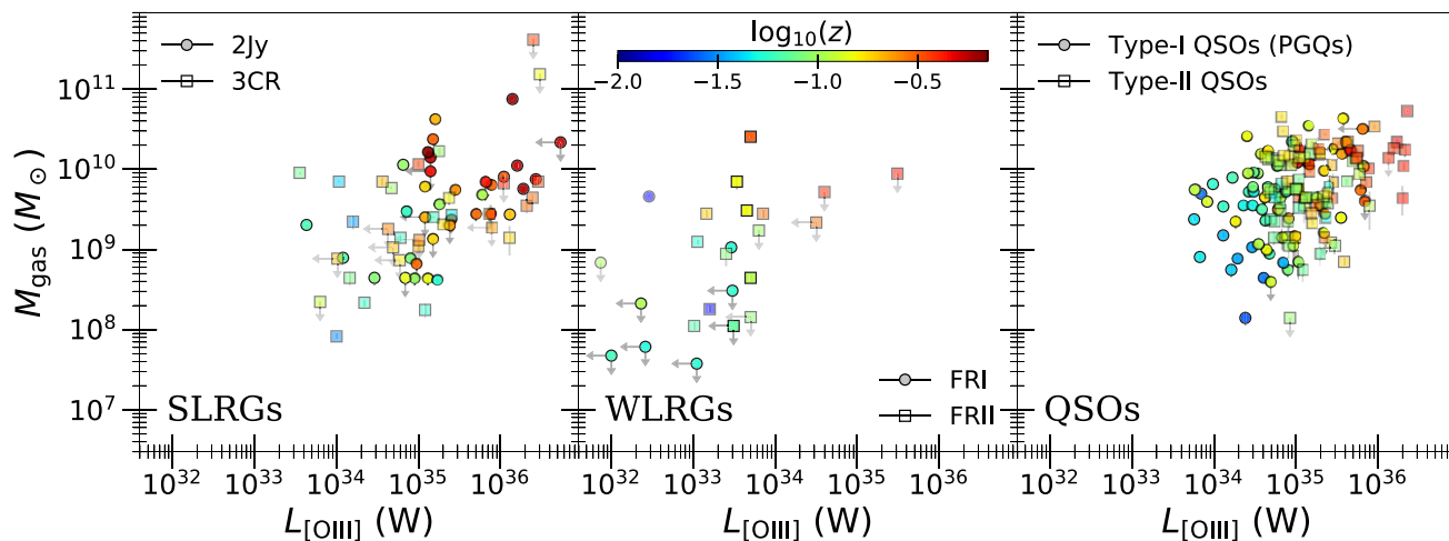
Figure 6. The cool ISM masses of our samples of AGNs versus L_{[\text{O III}]} , a proxy of AGN power. In reading order, we have the SLRGs, split in terms of the 2Jy and 3CR samples, the WLRGs, split in terms of FRI and FRII radio morphologies, and the radio-quiet QSOs, split in terms of Type-I (PGQs) and Type-II AGNs. Arrows indicate upper limits. The colour code indicates redshift, as shown by the colour bar at the top of the central panel ( 0.01 < z < 0.7 ).
