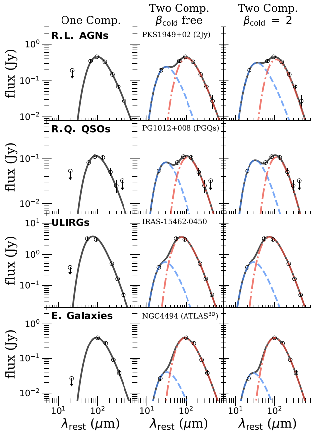
Figure 1. Examples of SED fits for one object of each of our populations of galaxies. From top-to-bottom, these are radio-loud AGNs, radio-quiet QSOs, ULIRGs, and non-AGN elliptical galaxies, as indicated in the top left-hand corner of each of the leftmost panels. The names of the sources and their respective samples selected to illustrate our SED fits are indicated at the top of each of the central panels. From left-to-right, the panels correspond to each of our three different models for the dust emission as described in Section 3.1.1. The observed fluxes are shown with open circles, and the best SED fits with a continuous black line. Downward arrows indicate upper limits on the fluxes. The warmer and the colder dust contributions are shown with a dashed blue line and a dot-dashed red line, respectively, for corresponding models. The full sets of SEDs and best-fitting parameters are available in the online material.
