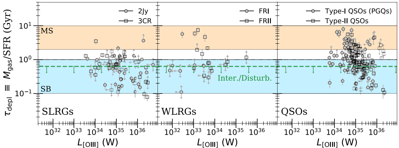
Figure 7. The depletion time-scales \tau_{\text{depl}} , measured as M_{\text{gas}}/\text{SFR} and expressed in Gyr, versus L_{[\text{OIII}]} (or AGN power) for our samples of SLRGs, WLRGs, and radio quiet QSOs (from left-to-right, respectively). We split the SLRGs into the 2Jy and 3CR samples, the WLRGs into FRIs and FRIIs, and the QSOs into Type-Is (PGQs) and Type-IIs (see keys). Arrows indicate upper and lower limits. The filled orange and blue areas indicate the range of \tau_{\text{depl}} typically observed in star-forming (MS) and starbursting (SB) galaxies, respectively (Kennicutt 1998). The horizontal dashed green line with downward arrows shows the \tau_{\text{depl}} below which most of interacting galaxies are expected to be found, as taken from Saintonge et al. (2012).
