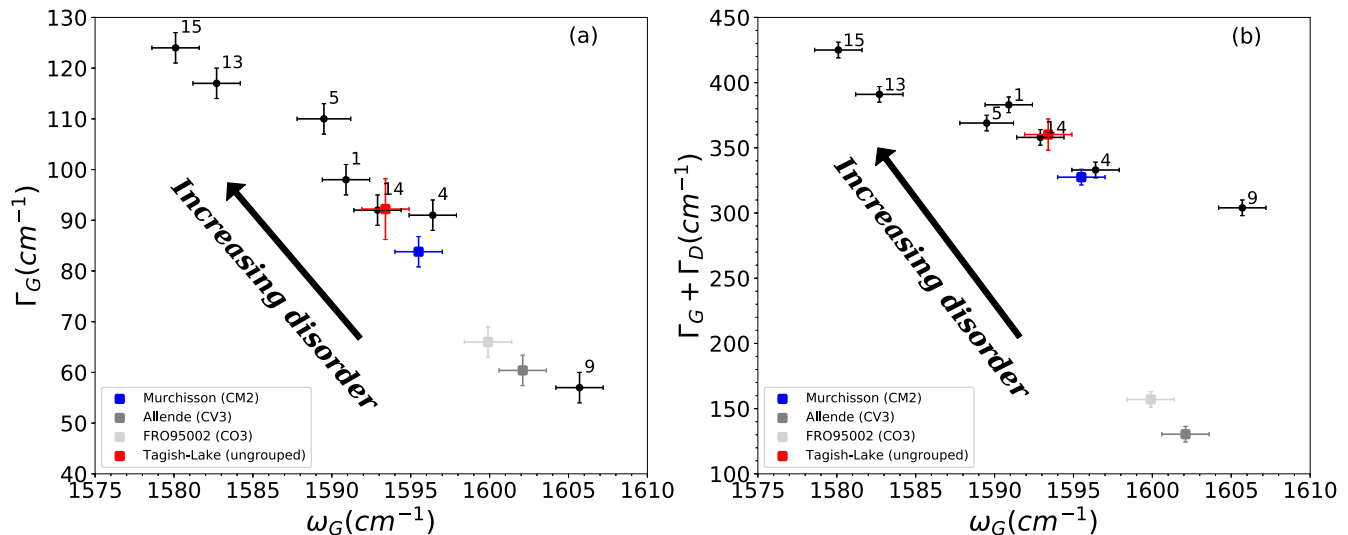
Figure 4. Panel (a) \Gamma_G as a function of \omega_G for the studied IDPs (represented by the black points and their corresponding allocated number), and the meteorites Murchisson (blue square), Allende (gray square), Tagish Lake (red square), and FRO95002 (light gray square). Panel (b) \Gamma_G + \Gamma_D in function of \omega_G for IDPs (black points), Murchisson (blue square), Allende (gray square), Tagish Lake (red square), and FRO95002 (light gray square) meteorites.
