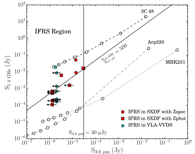
Figure 3. The locations of our IFRSs in the S_{1.4\text{ GHz}} versus S_{3.6\text{ }\mu\text{m}} diagnostic plot in which evolutionary tracks are shown for 3C 48 (dashed line), Arp 220 (dash-dotted line) and Mrk 231 (dotted line). The open circles represent redshifted data points with increasing redshift value from right to left, such that the first open circle having the highest flux on any track represents the current redshift of the source, the second circle represents the source placed at z = 1 , the third circle represents the source at z = 2 , and so on up to z = 7 . The vertical and diagonal solid lines represent our IFRS selection criteria S_{3.6\text{ }\mu\text{m}} < 30 \mu\text{Jy} and S_{1.4\text{ GHz}}/S_{3.6\text{ }\mu\text{m}} \geq 500 , respectively. The sources above the S_{1.4\text{ GHz}}/S_{3.6\text{ }\mu\text{m}} = 500 line are confirmed IFRSs, while the sources below this line are candidate IFRSs.
