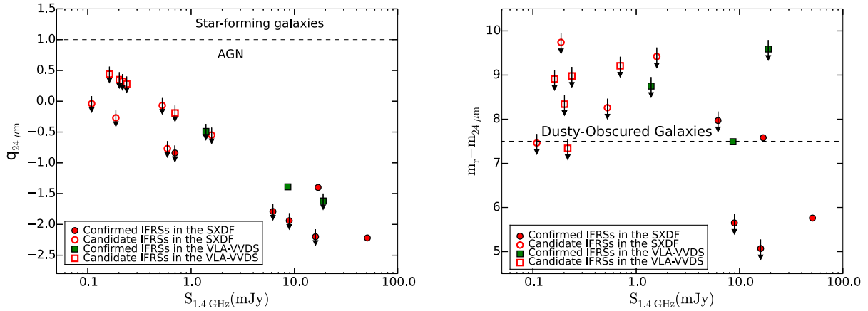
Figure 7. Left panel: q_{24} = \log(S_{24 \mu\text{m}}/S_{1.4\text{GHz}}) versus S_{1.4\text{GHz}} plot. Right panel: optical to 24- \mu\text{m} colour ( m_r - m_{24 \mu\text{m}} ) versus S_{1.4\text{GHz}} plot.
