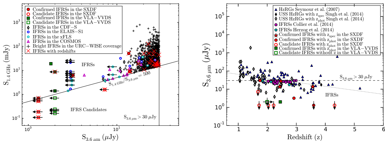
Figure 4. Left panel : S_{1.4 \text{ GHz}} versus S_{3.6 \mu\text{m}} plot for IFRSs from different samples. The solid lines mark IFRS selection criteria. The horizontal arrows depict upper limits on 3.6- \mu\text{m} fluxes. Right panel : S_{3.6 \mu\text{m}} versus redshift plot for IFRSs and H z RGs from different samples. The horizontal dashed line marks one of the selection criteria ( S_{3.6 \mu\text{m}} < 30 \mu\text{Jy} ) for IFRSs. The dotted line represents the linear regression line for all confirmed IFRSs and H z RGs. Downward arrows represent the upper limits on 3.6- \mu\text{m} fluxes. For the Collier et al. (2014) IFRS sample, 3.4- \mu\text{m} flux instead of 3.6- \mu\text{m} flux is available from the WISE survey.
