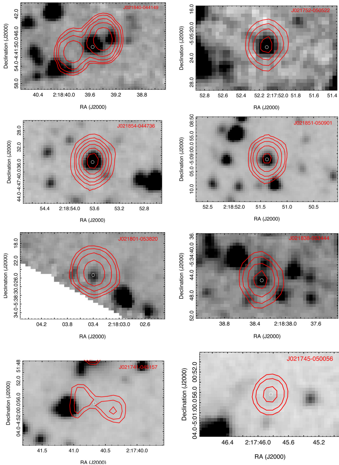
Figure A1. 1.4-GHz radio contours of our IFRSs overlaid on to 3.6- \mu m grey-scale images. The outermost first radio contour begins at 5\sigma with successive contour levels increased by a factor of \sqrt{2} . White circles represent the radio positions of the IFRSs.
