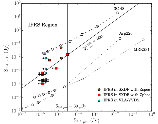
Figure 3. The locations of our IFRSs in the S_{1.4\text{GHz}} versus S_{3.6\mu\text{m}} diagnostic plot in which evolutionary tracks are shown for 3C 48 (dashed line), Arp 220 (dash-dotted line) and Mrk 231 (dotted line). The open circles represent redshifted data points with increasing redshift value from right to left, such that the first open circle having the highest flux on any track represents the current redshift of the source, the second circle represents the source placed at z = 1 , the third circle represents the source at z = 2 , and so on up to z = 7 . The vertical and diagonal solid lines represent our IFRS selection criteria S_{3.6\mu\text{m}} < 30 \mu\text{Jy} and S_{1.4\text{GHz}}/S_{3.6\mu\text{m}} \geq 500 , respectively. The sources above the S_{1.4\text{GHz}}/S_{3.6\mu\text{m}} = 500 line are confirmed IFRSs, while the sources below this line are candidate IFRSs.
