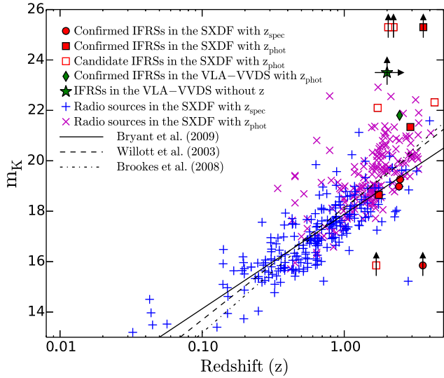
Figure 2. The locations of our IFRSs in the K - z plot displaying the radio sources detected in the SXDF (see Simpson et al. 2012). The vertical and horizontal arrows indicate lower limits on the K -band magnitudes and redshifts, respectively. Two IFRSs fall outside the UDS footprint and the lower limits ( m_K \geq 15.85 ) for these two IFRSs are from 2MASS. In the VLA-VVDS field, there are seven IFRSs with no redshift and no K -band magnitude, and such sources are placed at z > 2.0 based on the trend of the K - z relation and the K -band magnitude lower limits ( m_K \geq 23.5 from the VIDEO). The solid, dashed and dash-dotted lines represent the K - z relations for the samples of radio galaxies from Bryant et al. (2009), Willott et al. (2003) and Brookes et al. (2008), respectively.
