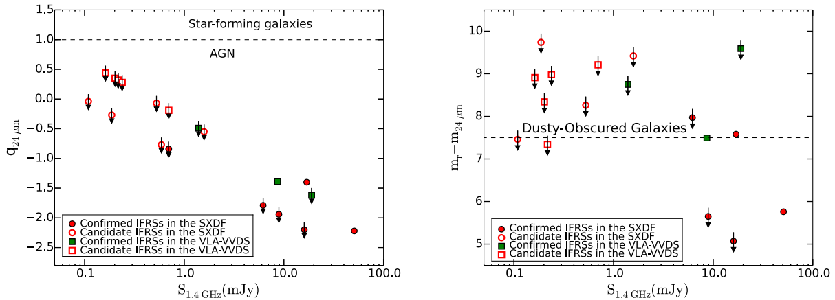
Figure 7. Left panel: q_{24} = \log(S_{24 \mu\text{m}}/S_{1.4 \text{ GHz}}) versus S_{1.4 \text{ GHz}} plot. Right panel: optical to 24-μm colour ( m_T - m_{24 \mu\text{m}} ) versus S_{1.4 \text{ GHz}} plot.
