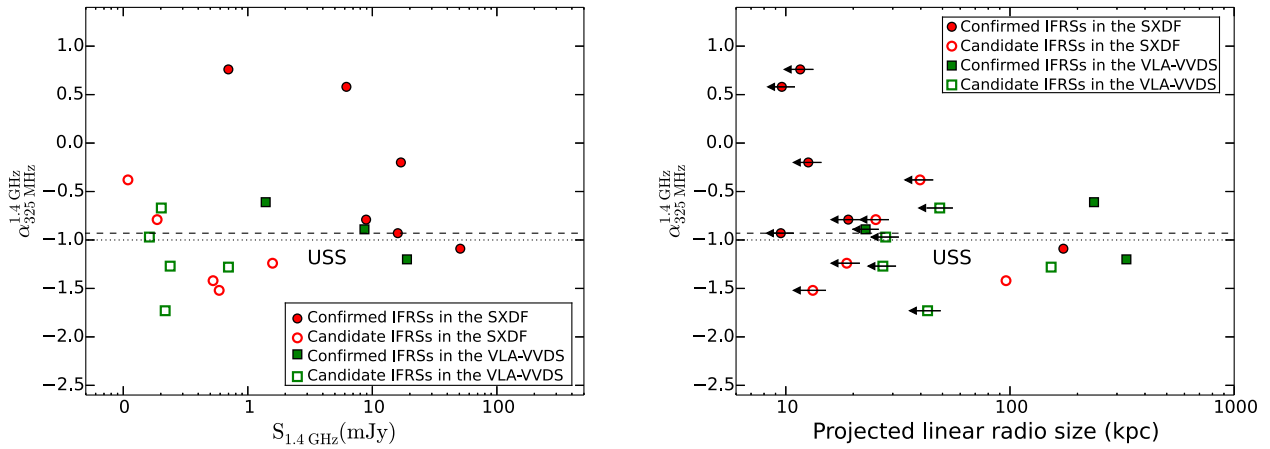
Figure 6. Left panel: \alpha_{325\text{MHz}}^{1.4\text{GHz}} versus S_{1.4\text{GHz}} plot. Right panel: \alpha_{325\text{MHz}}^{1.4\text{GHz}} versus radio size plot. Error bars are small and are of the order of the sizes of symbols. The horizontal dashed and dotted lines represent the median value ( \alpha_{325\text{MHz}}^{1.4\text{GHz}} = -0.93 ) of the spectral index distribution and the USS limit ( \alpha_{325\text{MHz}}^{1.4\text{GHz}} = -1.0 ), respectively.
