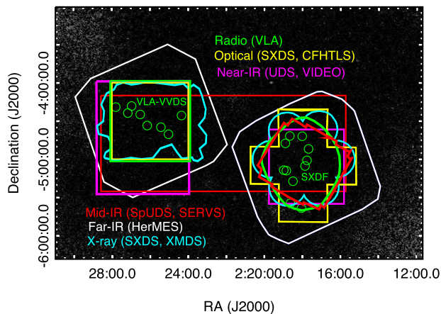
Figure 1. The footprints of deep multiwavelength surveys (i.e. 1.4-GHz radio in green, optical in yellow, NIR in magenta, MIR in red, FIR in white and X-ray in cyan) in the SXDF (right side) and VLA-VVDS (left side) overlaid on a part of the 325-MHz GMRT image. The footprints of large area surveys (i.e. SWIRE and 325-MHz GMRT) that cover both the deep fields are not shown here. The positions of our IFRSs are indicated by green circles.
