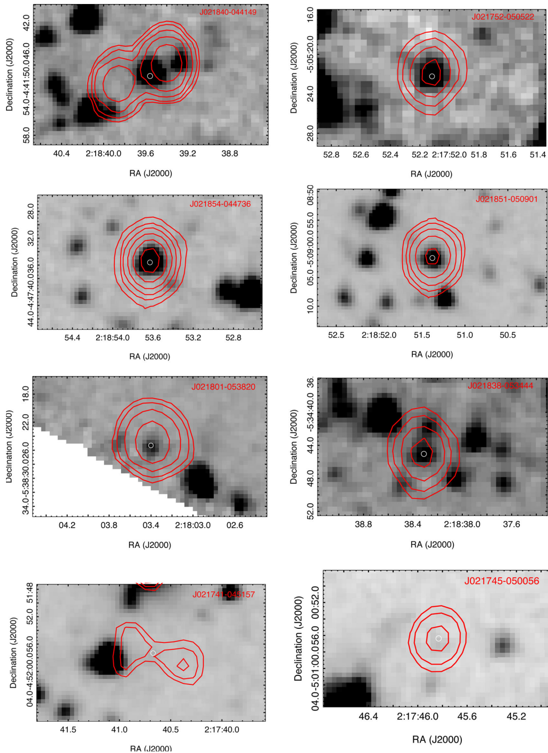
Figure A1. 1.4-GHz radio contours of our IFRSs overlotted on to 3.6- \mu m grey-scale images. The outermost first radio contour begins at 5\sigma with successive contour levels increased by a factor of \sqrt{2} . White circles represent the radio positions of the IFRSs.
