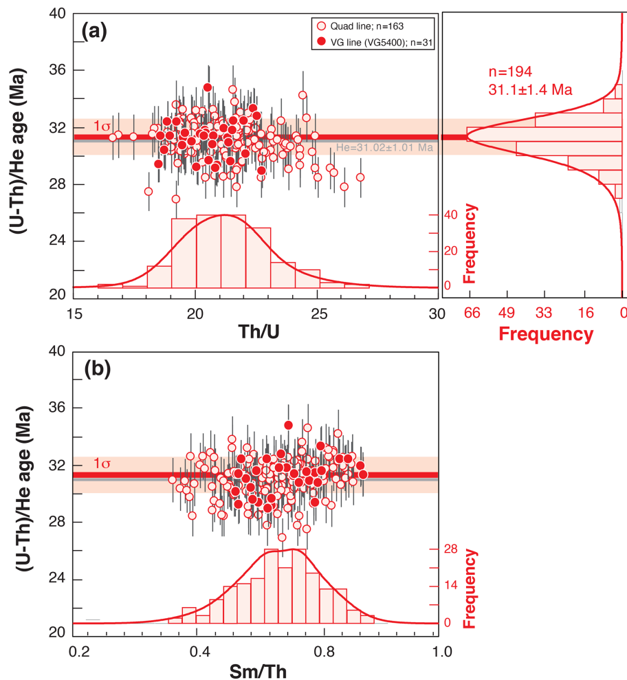
Figure 8. Durango (U–Th) / He age dispersion ( 1\sigma shown) as a function of Th / U (a) or Sm / Th ratios (b). Durango AHe ages and elemental ratios acquired from March to December 2019 using the quad line (open red circles) or the VG line (filled red circles). Histogram representation of the He ages; Th / U and Sm / Th ratios were constructed using RadialPlotter (Vermeesch, 2009). Th / U and Sm / Th ratios have no unit but are expressed by mass ( \text{ng ng}^{-1} ).
