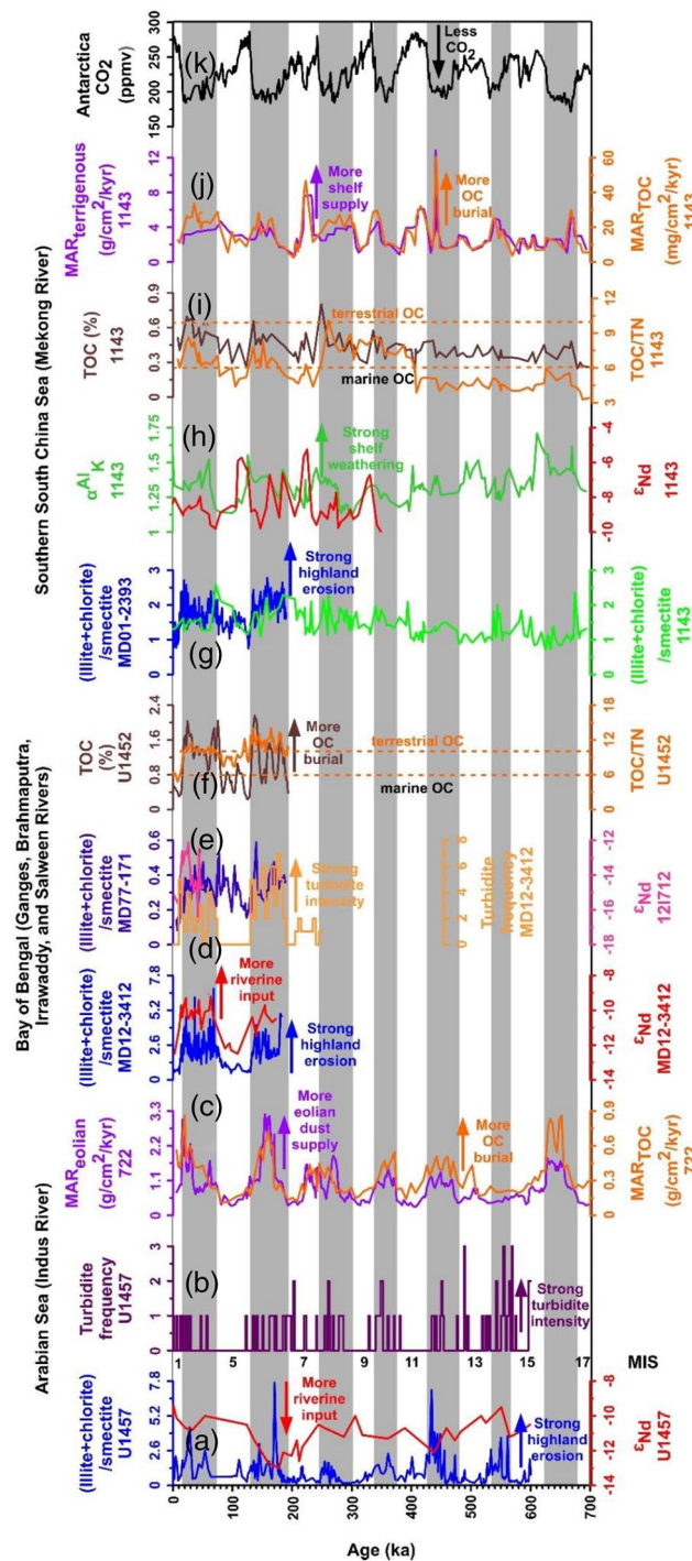
Figure 4. Comparison among (a) physical erosion in the Himalaya and Tibetan Plateau and the produced detritus supply (Yu et al., 2019), (b) turbidite frequency (Yu et al., 2019), and (c) mass accumulation rates of eolian dust ( MAR_{eolian} ) and total organic carbon ( MAR_{TOC} ; Clemens et al., 1996) in the deep Arabian Sea; (d) and (e) physical erosion in the Himalaya and Tibetan Plateau and the produced detrital input (Joussain et al., 2016; Liu et al., 2019; Yu et al., 2020), (f) turbidite frequency (Fauquembergue et al., 2019), and (g) physical erosion in the Himalaya and Tibetan Plateau and on the continental shelf (Liu et al., 2004; Wan et al., 2017), (h) and (i) chemical weathering on the continental shelf and supplies of the produced detritus and organic carbon, respectively (Wan et al., 2017; Wang et al., 2005), (j) mass accumulation rate of terrigenous detritus ( MAR_{terrigeneous} ; Wan et al., 2017), and (i) and (j) deposition of organic carbon in the distal southern South China Sea since ~400 ka (Wang et al., 2005); and (k) atmospheric CO_2 concentration from the Antarctic Dome C ice cores (Luthi et al., 2008). MIS = marine isotope stage. \alpha_{Al-K} = (Al/K)_{sample}/(Al/K)_{upper\ continental\ crust} . Note the unique values of almost all of the proxies during sea-level lowstands (gray bars).
