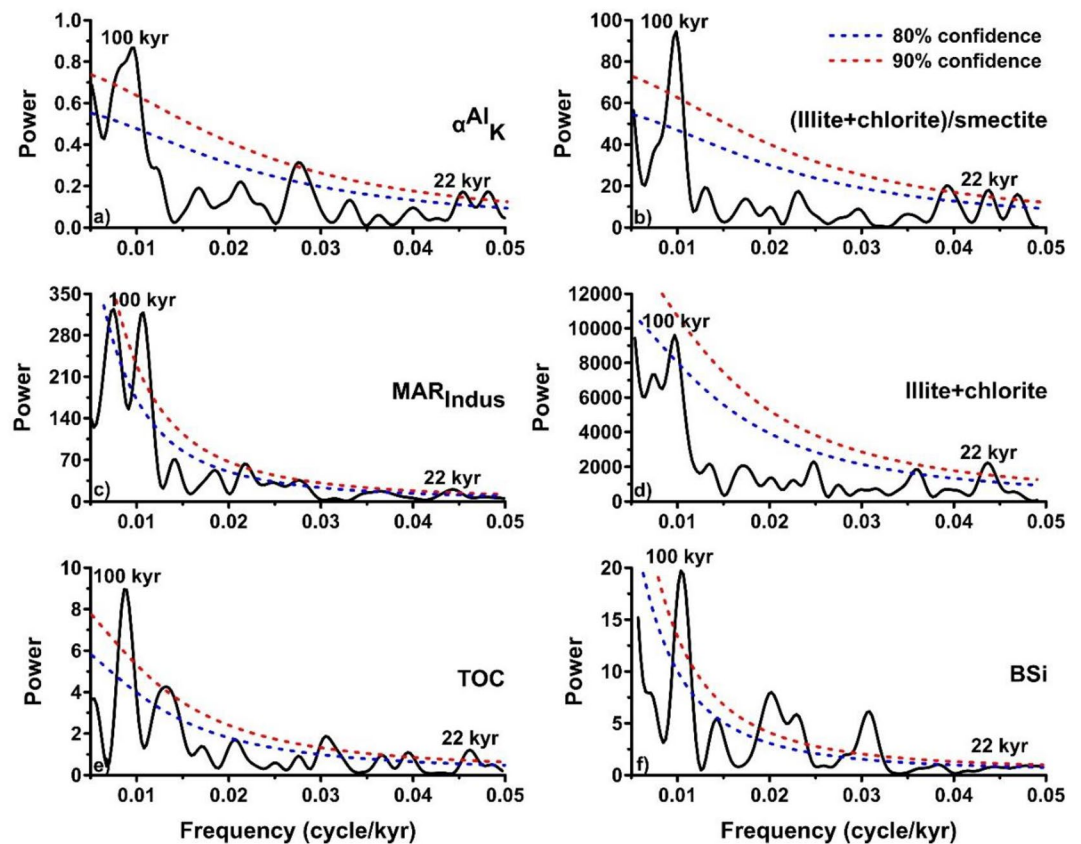
Figure 3. Frequency analyses of some typical proxies at IODP Site U1456, showing the primary orbital periodicities (eccentricity of 100 kyr and precession of 22 kyr) since ~700 ka (Cai et al., 2018, 2019; Chen, Xu et al., 2019, 2020). \alpha_{Al_K}^{Al} = (Al/K)_{sample}/(Al/K)_{upper\ continental\ crust} . MAR_{Indus} = mass accumulation rate of the Indus River detritus. TOC = total organic carbon. BSi = biogenic silica.
