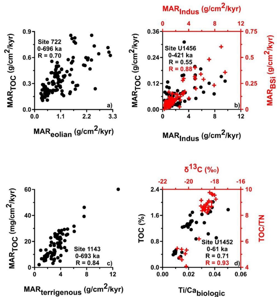
Figure 5. Cross plots of some typical proxies from the representative sediment cores in the study area. R = correlation coefficient. MAR_{eolian} = mass accumulation rate of eolian dust. MAR_{TOC} = mass accumulation rate of total organic carbon. MAR_{Indus} = mass accumulation rate of the Indus River detritus. MAR_{BSi} = mass accumulation rate of biogenic silica. MAR_{terrigeneous} = mass accumulation rate of terrigenous detritus. Ti/Ca_{biologic} = ratio of Ti to biologic Ca. TOC = total organic carbon. TOC/TN = ratio of total organic carbon to total nitrogen.
