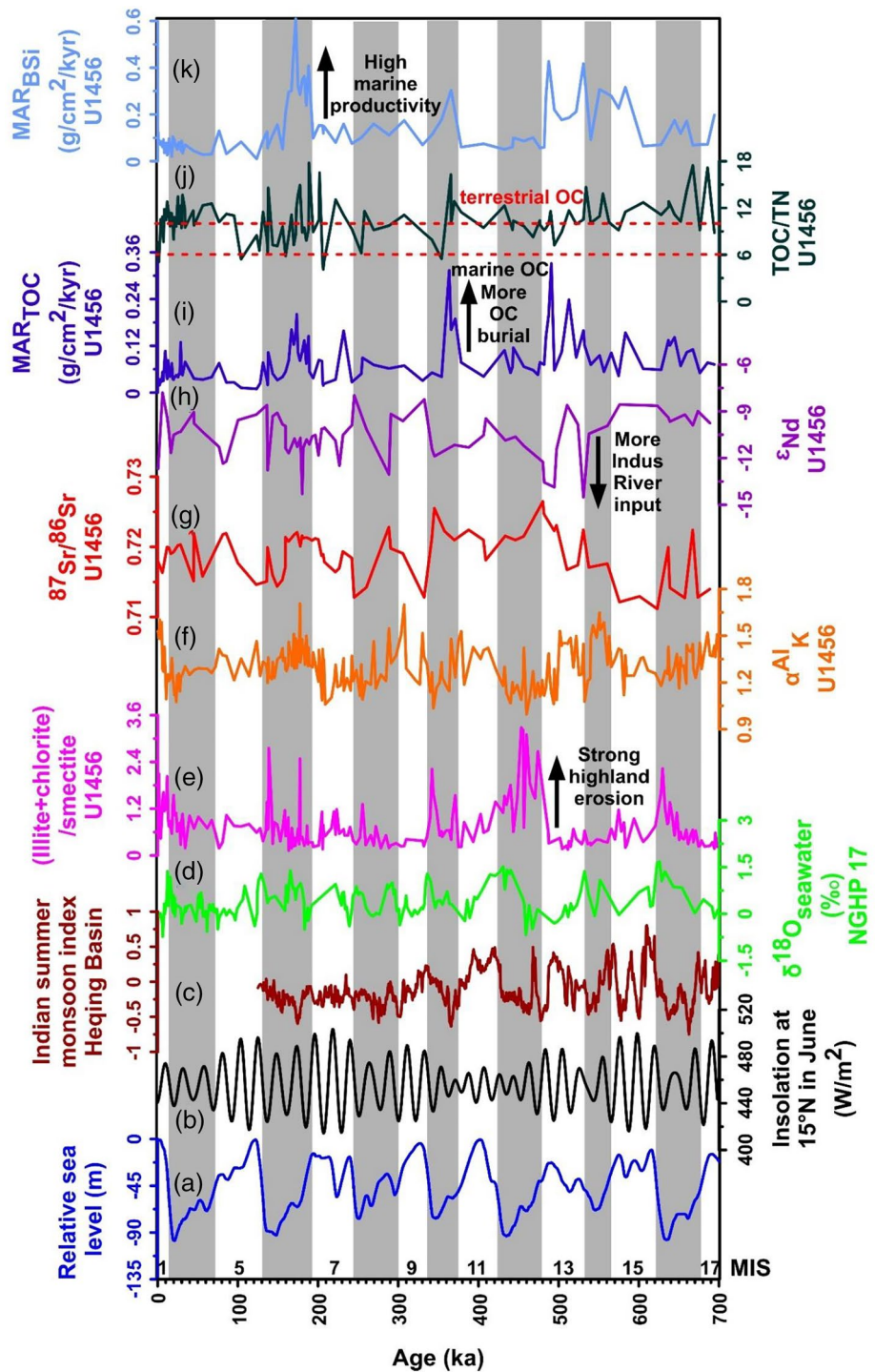
Figure 2. Comparison among (e) (illite + chlorite)/smectite ratio (Cai et al., 2018; Chen, Xu, et al., 2019), (f) (Al/K)_{sample}/(Al/K)_{upper\ continental\ crust} ratio ( \alpha_{AlK} ; Cai et al., 2019; Chen et al., 2020), (g) ^{87}Sr/^{86}Sr ratio (Cai et al., 2019; Chen et al., 2020; Khim et al., 2018), (h) \epsilon_{Nd} (Cai et al., 2019; Chen et al., 2020; Khim et al., 2018), (i) mass accumulation rate of total organic carbon ( MAR_{TOC} ), (j) ratio of total organic carbon to total nitrogen (TOC/TN), and (k) mass accumulation rate of biogenic silica ( MAR_{BSi} ) at IODP Site U1456, as well as (a) relative sea level (Bintanja et al., 2005), (b) insolation calculated at 15°N in June (Berger & Loutre, 1991), (c) Indian summer monsoon index of the Heqing Basin (An et al., 2011), and (d) \delta^{18}O value of seawater from Core NGHP 17 (Gebregiorgis et al., 2018). MIS = marine isotope stage. OC = organic carbon. Note the unique values of almost all of the proxies during sea-level lowstands (gray bars).
