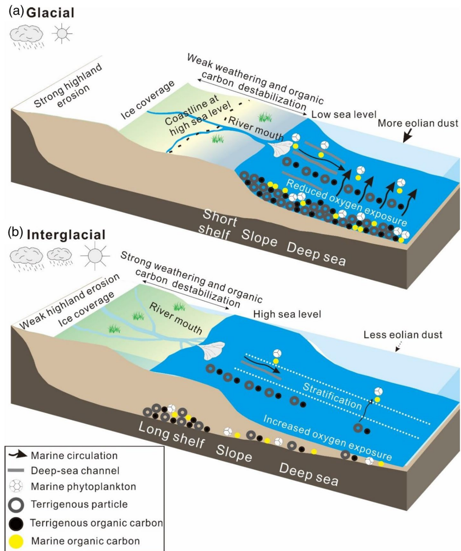
Figure 6. Schematic model of processes associated with physical erosion in the Himalaya and Tibetan Plateau and transport of the produced detritus and organic matter, eolian dust input, hydrological dynamics, marine productivity, and organic carbon burial in the Arabian Sea and Bay of Bengal during (a) glacial and (b) interglacial periods, derived from both the current study and previous research (e.g., An et al., 2011; Chen et al., 2019a 2019b; Clemens et al., 1996; Fauquembergue et al., 2019; Hein et al., 2020; Kim et al., 2018; Lee et al., 2020; Liu et al., 2019; Ramaswamy et al., 2008; Weber et al., 2018; Yu et al., 2019).
