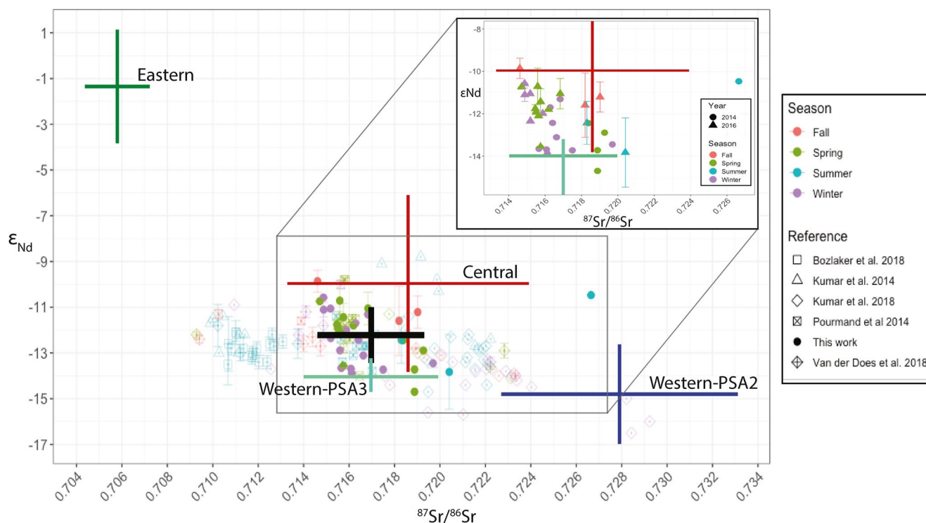
Figure 2. Results showing the ^{87}\text{Sr}/^{86}\text{Sr} and \epsilon_{\text{Nd}} isotopic signature of samples collected in South America (This work; filled circles). The green, red, blue, and turquoise crosses correspond to the average ^{87}\text{Sr}/^{86}\text{Sr} and \epsilon_{\text{Nd}} and one standard deviation ( \pm 1\text{SD} ) and correspond to the source locations (potential source areas [PSAs]) shown in Figure 1. The isotopic signature of the Eastern, Central, and Western-PSA2 were adapted following Jewell et al. (2020). Due to the lack of samples from the Western-PSA3, its isotopic signature was inferred from samples collected nearby in Cape Verde (Kumar et al., 2018) and Mbour, Senegal (Skonieczny et al., 2013). The black cross shows the average and \pm 1\text{SD} of our data. Data from previously published literature of dust collected at receptor sites are shown in unfilled markers with colors that correspond to the season in which they were collected. Error bars on data points represent \pm 1\text{SD} , except for Pourmand et al. (2014) and this study, which shows 95% confidence intervals. When error bars are not present, SDs are smaller than their marker size. Winter is DJF, spring is MAM, summer is JJA, and fall is SON. The insert shows the section of the plot inside the gray box and further subdivides our data by year.
