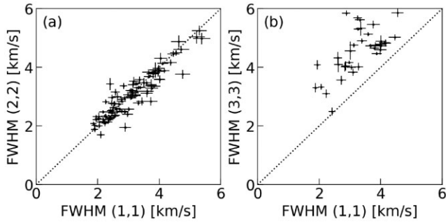
Figure 3 Scatter plots of FWHM linewidth of \text{NH}_3 (1,1), (2,2), and (3,3) emission. The solid lines indicate the line of equality.
