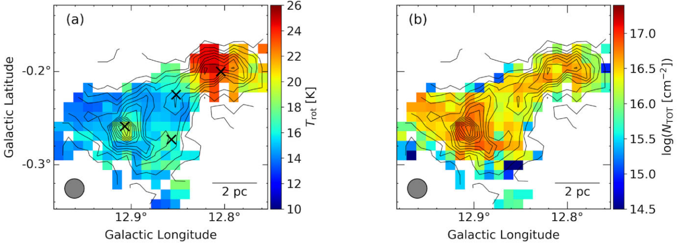
Figure 4. Spatial distributions of the physical parameters described in Section 3.3. The plotted values are representative along the velocity axis. (a) The rotational temperature; (b) the total column density of \text{NH}_3 gas. Contours indicate the \text{NH}_3(1,1) integrated intensity map, which is the same as in Fig. 2(a). The NRO45 beam size is indicated by the grey circle shown in the lower left corner of each panel. Cross marks are the same as inside the dashed rectangle in Fig. 1(a).
