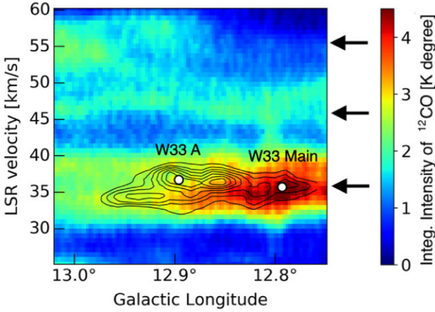
Figure 6. Longitude-velocity diagram of the ^{12}\text{CO} ( J=1-0 ) emission using FUGIN data (colour image) and the \text{NH}_3(1,1) main line emission (contour). The white circles indicate the peak velocities of W33 A and W33 Main in the \text{C}^{18}\text{O} ( J=1-0 ) emission line (Umemoto et al. 2017; Kohno et al. 2018). The arrows show the three velocity components at 35, 45, and 55 \text{km s}^{-1} . The lowest contour level and contour intervals are 0.06 K degree and 0.03 K degree, respectively.
