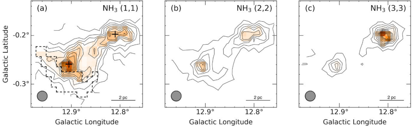
Figure 2. Integrated intensity map of \text{NH}_3 : (a) (1,1), (b) (2,2), and (c) (3,3). The NRO45 beam size is indicated by the grey circle shown in the lower left corner of each panel. The lowest contour and contour steps are 20\sigma ( 0.8 \text{ K km s}^{-1} ) in T_a^* , respectively. Plus marks indicate the positions of \text{H}_2\text{O} maser emission. The black dashed enclosure shows the region where double-peak profiles were detected.
