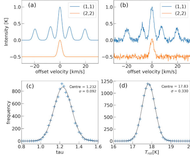
Figure A2. The result of error estimation with our method. (a) Model profiles of \text{NH}_3 (1,1) (blue) and (2,2) (orange); (b) profiles with Gaussian noise (rms 0.04 K) added to the model profile shown in (a); (c) and (d) frequency distributions of the optical depth and rotational temperature, respectively. The black line shows the best-fitting log-normal function.
