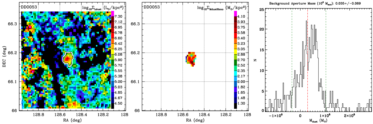
Figure 18. DDO 053: Left: \Sigma_{Ld} map; contours: \Sigma_{Ld,min} = 0.6 L_{\odot} \text{pc}^{-2} . Center: \Sigma_{Md} map within the galaxy mask. Right: histogram of M_d for H I-based mask, shifted randomly. Red dotted–dashed line: M_d for mask centered on galaxy. 68% of random masks give M_d between green dashed lines. (The complete figure set (8 images) is available.)
