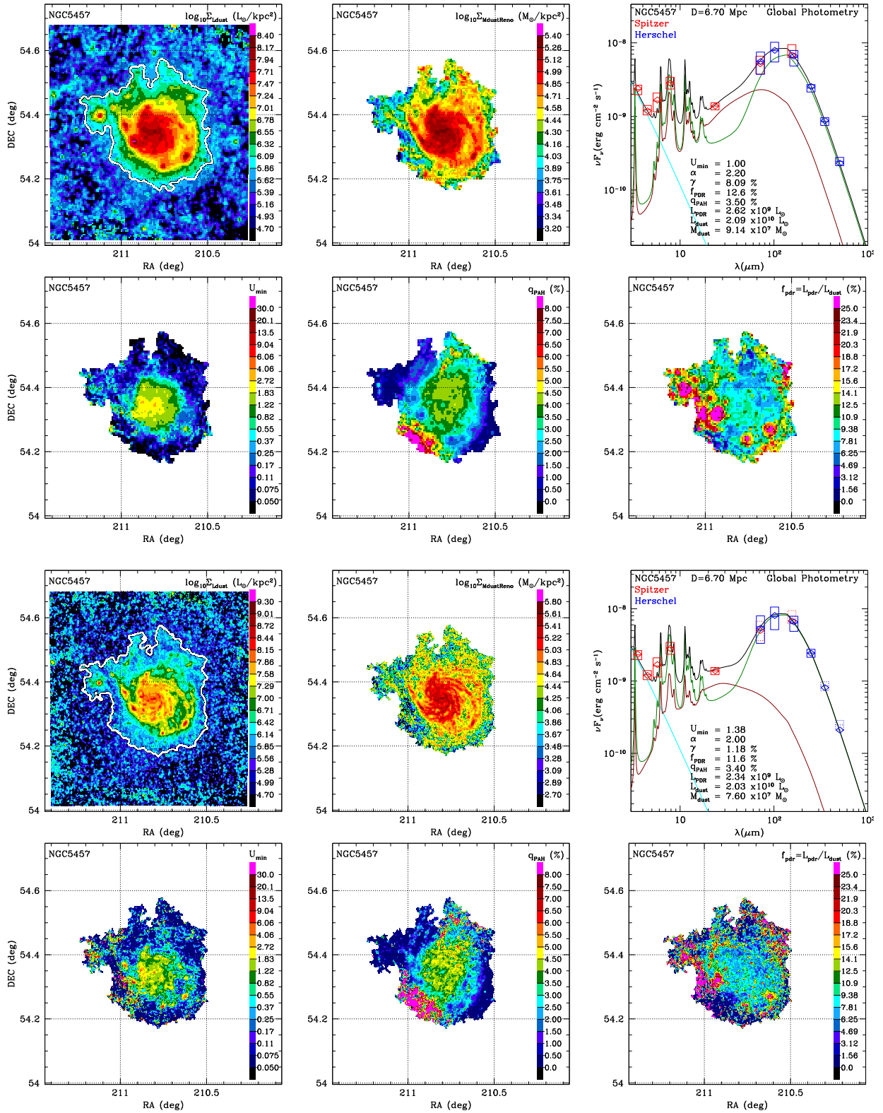
Figure 5. NGC 5457 = M101: model results at M160 PSF (rows 1 and 2) and at S250 PSF (rows 3 and 4). Dust luminosity per area \Sigma_{Ld} (column 1, rows 1 and 3) is shown for the entire field, with the adopted galaxy mask boundary in white. Dust mass per area \Sigma_{Md} (column 2, rows 1 and 3) is after renormalization (see text). U_{\text{min,DL07}} , q_{\text{PAH}} , and f_{\text{PDR}} are shown in rows 2 and 4. The global SED (column 3, rows 1 and 3) is shown for single-pixel modeling, with contributions from dust heated by U_{\text{min}} (green), dust heated by U > U_{\text{min}} (red), and starlight (cyan); values of U_{\text{min}} and M_d in the figure label are for the DL07 model before renormalization. Herschel (blue rectangles) and Spitzer (red rectangles) photometry is shown. Diamonds show the band-convolved flux for the model. The horizontal extent of rectangles and diamonds is an arbitrary \pm 10\% wavelength range. The vertical extent of photometry rectangles is \pm 1\sigma .
