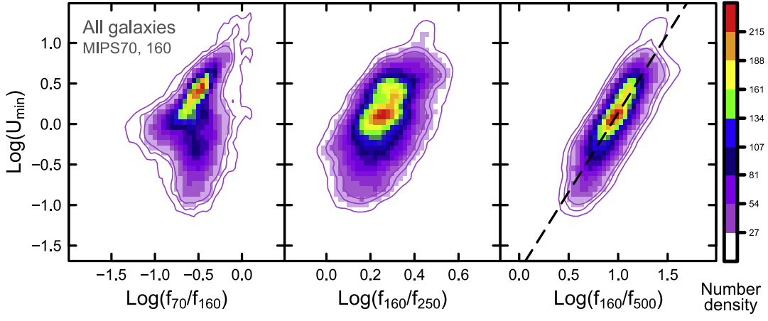
Figure 12. Minimum starlight heating intensity U_{\min} versus f_{70}/f_{160} (left panel), f_{160}/f_{250} (middle), and f_{160}/f_{500} (right) for all galaxies. The 70 and 160 \mu\text{m} flux densities f_{70} and f_{160} are from MIPS only (see text). The color coding corresponds to number density of pixels, as shown by the rightmost color bar. The left panel shows that f_{70}/f_{160} is not a good indicator of U_{\min} , because f_{70} is sensitive to both single-photon heating and the emission from dust exposed to starlight intensities U > U_{\min} . The middle panel with f_{160}/f_{250} avoids using f_{70} , but the wavelength range is insufficient to adequately sample U_{\min} and a luminosity-weighted dust temperature. Instead, the right panel shows the tight correlation between U_{\min} and f_{160}/f_{500} (the dashed line is Equation (22)), illustrating the close relationship between the minimum heating intensity and the coolest dust.
