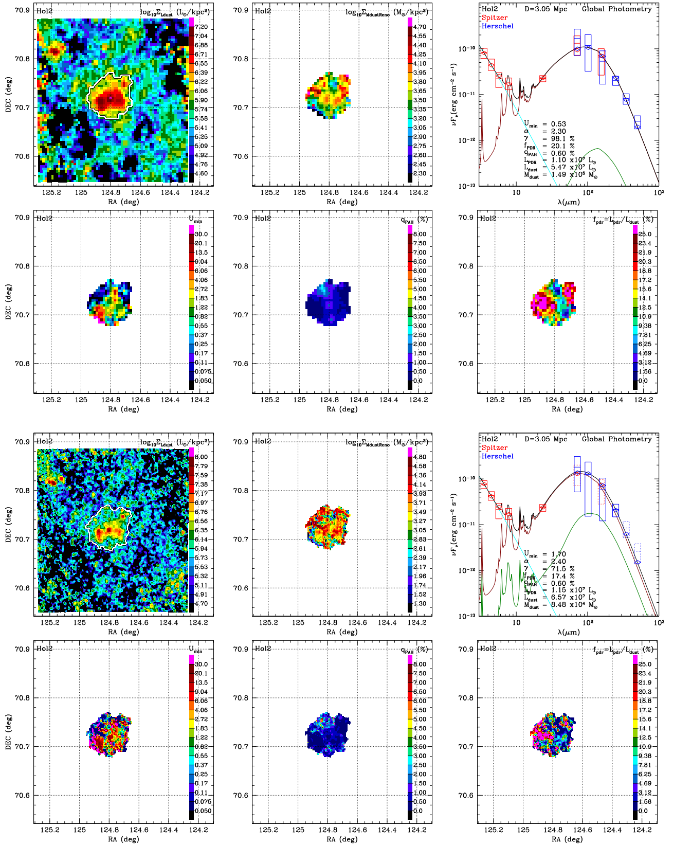
Figure 17. HoI2: Model results at M160 PSF (rows 1 and 2) and at S250 PSF (rows 3 and 4). Dust luminosity per area \Sigma_{Ld} (column 1, rows 1 and 3) is shown for the entire field, with the adopted galaxy mask boundary in white. Dust mass per area \Sigma_{Md} (column 2, rows 1 and 3) is after renormalization (see text). U_{\min} , f_{\text{PAH}} , and f_{\text{PDR}} are shown in rows 2 and 4. The global SED (column 3, rows 1 and 3) is shown for single-pixel modeling, with contributions from dust heated by U_{\min} (green) and dust heated by U > U_{\min} (red) and starlight (cyan); values of U_{\min} and M_d in the figure label are for the DL07 model before renormalization. Herschel (blue rectangles) and Spitzer (red rectangles) photometry is shown; the vertical extent is \pm 1\sigma . Diamonds show the band-convolved flux for the model.
