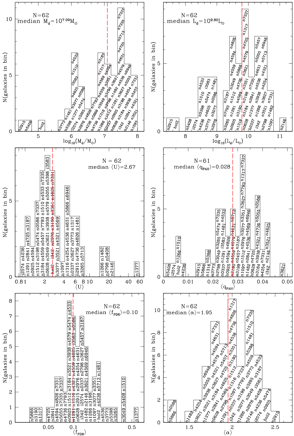
Figure 6. Distributions of dust and starlight parameters for the KF62 sample. NGC 1377 is omitted from the q_{PAH} histogram (see the text). M_d and \langle U \rangle are renormalized values.
