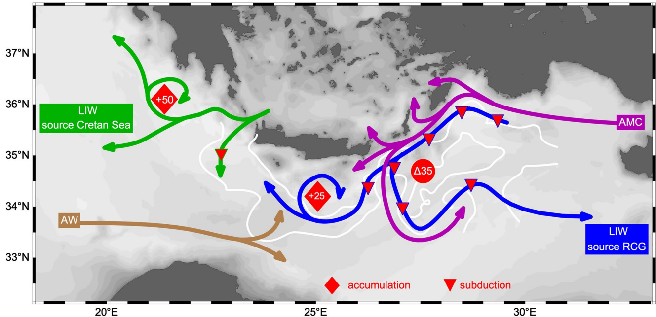
Figure 9. Schematic regional circulation inferred from multi-platform surveys between 15 October 2018 and 31 July 2019. The light and salty waters supplied by the AMC were transformed into LIW from two sources: the RCG and the Cretan Sea. AW was not observed in the two source regions. Part of LIW resulting from subduction in the periphery of the RCG was accumulated in the Cretan Passage. LIW resulting from the Cretan outflow was accumulated offshore the Peloponnese. Wintertime variations of LIW stocks indicated in meter per unit horizontal area. Locations of subduction (red triangles) and accumulation (red diamonds), dynamic contours -42 and -39 dyn cm (white lines).
