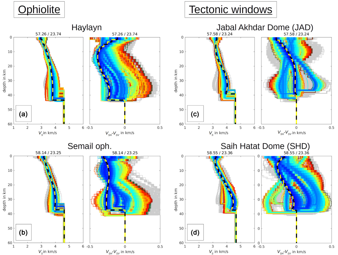
Figure 5. Inversion of local dispersion curve – Isotropic V_S and radial anisotropy. Each panel shows local 1-D model of isotropic V_S (left-hand panel) and radial anisotropy ( V_{SH}-V_{SV} ) (right-hand panel), sorted by decreasing misfit (red to blue, 5000 best-fitting models shown). Locations of points are shown as green squares in Fig. 1(a). (a) Batinah plain north of Haylayn ophiolite; (b) Semail ophiolite between JAD and SHD; (c) JAD and (d) SHD.
