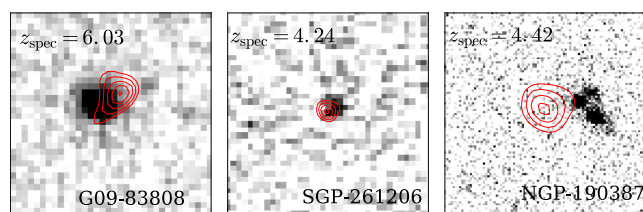
Figure 4. Near-IR (K-band) 11 \text{ arcsec} \times 11 \text{ arcsec} images of G09-83808 and SGP-261206 from VIKING survey (Edge et al. 2013) and NGP-190387 from Gemini/NIRI (programme GN-2016A-FT-32). Red contours represent the 1.3-mm (G09-83808, NGP-190387) and 3-mm (SGP-261206) continuum emission, at 5, 6, 7, 8, 9 \times \sigma . Near-IR emission is seen clearly, coincident or near-coincident with the 1.3- or 3-mm continuum emission. At the depth of the VIKING observations (limiting magnitude, K_{\text{AB}} \simeq 21.2 ), we do not expect to detect dust-obscured distant galaxies. The sources coincident with G09-83808 and SGP-261206 show, therefore, that these two DSFGs are amplified gravitationally by the foreground galaxies seen in the near-IR images. The galaxy in the foreground of SGP-83808 has z_{\text{spec}} = 0.778 , obtained using X-shooter on the VLT (Fig. 5), and is magnified by 8.2 \pm 0.3 , a factor determined using high-resolution ALMA continuum imaging (see Oteo et al., in preparation-a). The three galaxies revealed by the deeper Gemini imaging of NGP-190387 are considerably fainter, with K_{\text{AB}} = 21.0, 22.3, 21.4 , yet they are not coincident with the z = 4.42 DSFG and likely constitute a foreground lensing group.
