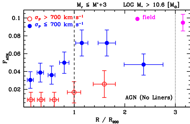
Figure 6. Variation of AGN fraction as a function of clustercentric distance for low ( \sigma_p \leq 700 \text{ km s}^{-1} ) mass clusters (displayed by blue filled circles) and high mass systems ( \sigma_p > 700 \text{ km s}^{-1} , red open circles). The corresponding estimate for the field is indicated by the magenta filled circle. The error bars indicate the 1\sigma standard error on the biweight location estimate. [A colour version of this figure is available in the online version.]
