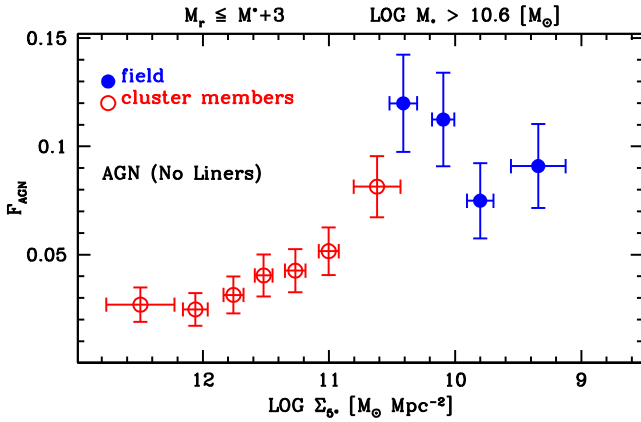
Figure 3. Dependence of AGN fraction as a function of local galaxy stellar mass density ( \Sigma_{5*} ), for cluster (red open circles) and field (blue filled circles) objects. The error bars indicate the 1\sigma standard error on the biweight location estimate. [A colour version of this figure is available in the online version.]
