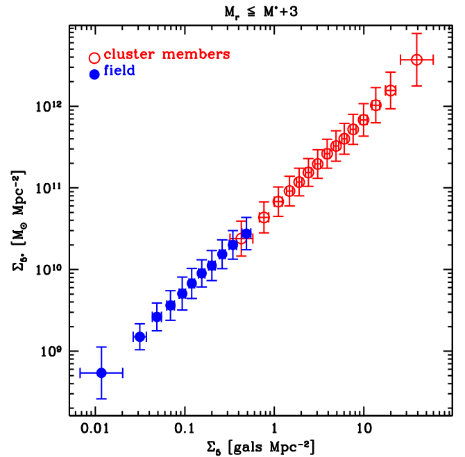
Figure 1. Comparison between the galaxy stellar mass density ( \Sigma_* ) and the galaxy number density ( \Sigma_g ), for cluster (red open circles) and field (blue filled symbols) galaxies. The error bars indicate the 1\sigma standard error on the biweight location estimate. [A colour version of this figure is available in the online version.]
