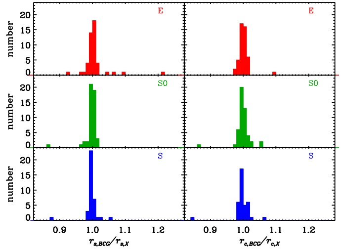
Fig. 7. Histogram distributions of the ratio of best-fit NFW (left panels) and King (right panels) model scale radius parameters for individual clusters, using BCG and X-ray centers, for the E, S0, and S populations in the top, middle, and bottom panels, respectively.
