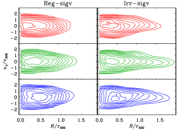
Fig. 3. Adaptive-kernel density maps in projected phase-space (rest-frame velocities versus distances from the cluster centers) for the Reg-sigv ( left panels ) and Irr-sigv ( right panels ) stacks. Radii and velocities are in normalized units, using r_{200, \sigma} and v_{200, \sigma} for the normalization of radii and velocities, respectively. Upper panel: E, middle panel: S0, lower panel: S. Density contours are space logarithmically.
