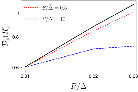
Figure 1. The density part of structure function for different dust absorption extent for shallow density with v_\rho = -1/2 , r_c/\bar{\Delta} = 0.01 , \sigma/\bar{\Delta} = 0.1 and v = 2/3 . The solid line is produced using the simplified model presented in equation (56), with just the density part. As shown in the figure, the density contribution flattens as dust absorption becomes strong.
