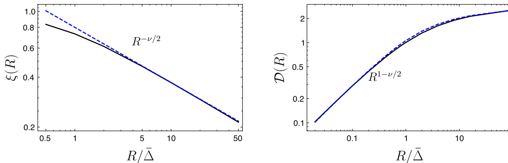
Figure 2. Left: intensity correlation function produced by full numerical integration for a thin slice case for steep density and velocity field, with spectral index v = 2/3 and v_\rho = 1/3 . The parameters used are \sigma_\rho/\bar{\rho} = 0.2 , r_c/\bar{\Delta} = S/\bar{\Delta} = 100 . Both velocity and density fluctuations are taken to following Gaussian distribution. Right: intensity structure function at different scales for the same parameters. The solid curve is produced using exact numerics [see Appendix A and equation (18)], while the dotted curve is produced by using equations (56) and (18), with S/\Delta_0 = 66 . At short R , the asymptote is R^{1-\nu/2} , while at larger lags, the structure function becomes saturated.
