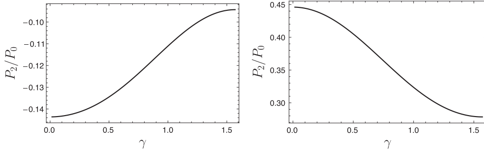
Figure 8. Low- \beta fast modes at M_A = 0.7 : quadrupole to monopole ratio of power spectrum of intensity fluctuations. Left-hand panel: the observed ratio in the case of negligible dust absorption or at scales K \gtrsim \Delta_0^{-1} . Right-hand panel: the observed ratio in the presence of dust absorption at scales K \lesssim \Delta_0^{-1} .
