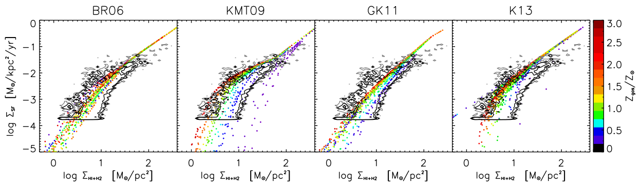
Figure 4. The star formation rate surface density against neutral gas surface density. Coloured dots are results of model galaxies at redshift z = 0 with different metallicities of the cold gas. Black contours show the distribution of observed galaxies from Bigiel et al. (2010, only points in the optical disc are included). Different star formation laws are shown in different panels.
