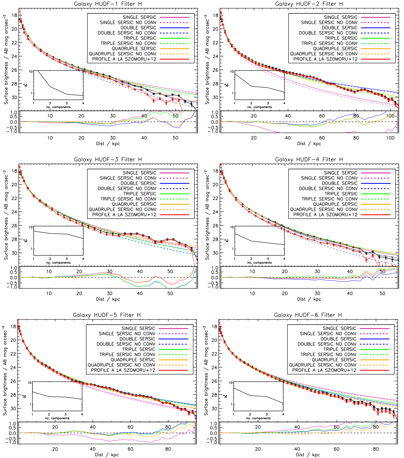
Figure A1. Observed (black line), model (convolved and non-convolved with the PSF, coloured solid and dashed lines, respectively, with colours indicated in the legend) and ‘a la Szomoru’ (deconvolved adding the residuals of the four Sérsic fit; red line) galaxy surface brightness profiles for our galaxy sample in the H band. The subplot shows the reduced chi-square ( \chi^2_r ) values for the Sérsic fits we performed. The bottom miniplots display the differences between the observed surface brightness profile and the multi-Sérsic PSF convolved models.
