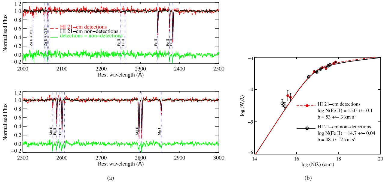
Figure 7. (a) The median stacked spectrum of SDSS quasars with strong Fe II systems at 0.5 < z < 1.5 (in rest frame) which are detected in H I 21-cm absorption is shown as the red dashed line, and the same for systems which are not detected in H I 21-cm absorption is shown as the black solid line. The difference of the stacked spectrum of H I 21-cm non-detections from that of the detections is shown as the green line at an arbitrary offset in the y-axis for clarity. The various rest wavelengths of transitions of Mg II, Mg I, Cr II, Mn II, Fe II and Zn II are marked by vertical dotted lines. (b) The COG for Fe II lines detected in the stacked spectrum of H I 21-cm detections is shown as the red dashed line and that for Fe II lines detected in the stacked spectrum of H I 21-cm non-detections is shown as the solid black line. The filled and open circles mark the observed rest-frame equivalent widths and the column densities calculated for Fe II lines in the stacked spectrum of H I 21-cm detections and non-detections, respectively.
