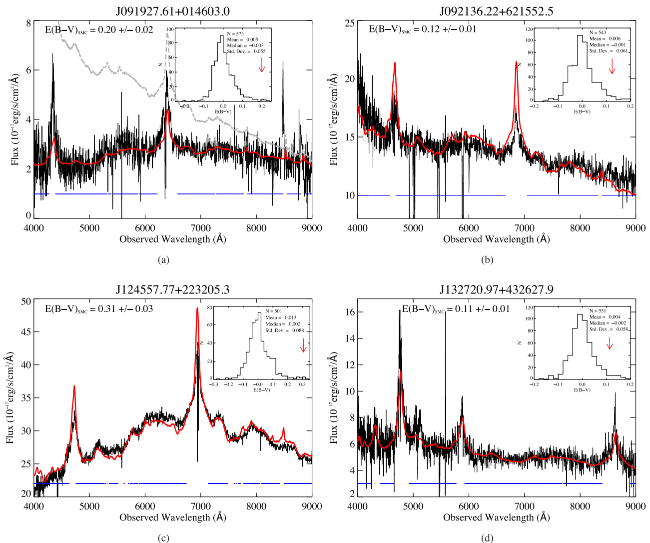
Figure 8. SED fit to the spectra of (a) J0919+0146, (b) J0921+6215, (c) J1245+2232 and (d) J1327+4326, taking into account the reddening by the intervening absorber. SMC extinction curve gives best fit to all of them. The best-fitting E(B - V) values are provided in each panel. The horizontal regions indicate the spectral range considered in the fitting process. Inset in each panel is the distribution of E(B - V) for a control sample of SDSS quasars (see Section 7.1 for details). The number of quasars, mean, median and standard deviation of E(B - V) in the control sample are also provided. The arrows indicate the E(B - V) values obtained for the respective quasars. The unreddened SDSS quasar composite spectrum (Vanden Berk et al. 2001) is shown as the grey dashed line in panel (a).
