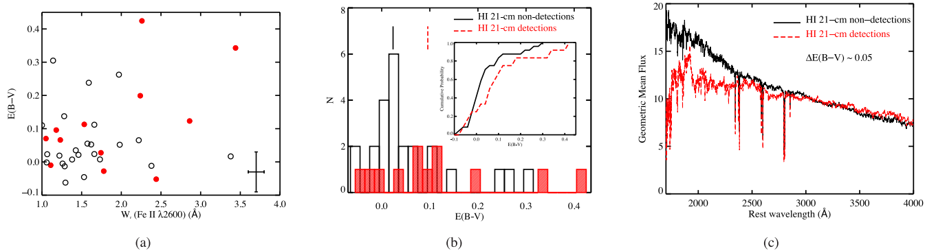
Figure 9. (a) E(B - V) versus W_{\text{Fe II}} for the strong \text{Fe II} systems. Filled symbols correspond to \text{H I} 21-cm detections and open symbols correspond to non-detections. The typical error bars are plotted in the bottom right corner. (b) The histogram distributions of E(B - V) values for strong \text{Fe II} systems that show \text{H I} 21-cm absorption (red shaded) and those which do not (black open). The inset shows the cumulative distributions of E(B - V) for systems with and without \text{H I} 21-cm absorption as red dashed and black solid lines, respectively. The vertical dashed and solid ticks mark the median E(B - V) for systems with and without \text{H I} 21-cm absorption, respectively. (c) The geometric mean stacked spectrum of SDSS quasars with strong \text{Fe II} systems at 0.5 < z < 1.5 (in rest frame) which are detected in \text{H I} 21-cm absorption is shown as the red dashed line, and the same for systems which are not detected in \text{H I} 21-cm absorption is shown as the black solid line. The spectra have been smoothed by 5 pixels for display purpose. The differential reddening, \Delta E(B - V) , is indicated in the figure (see Section 7.2 for details).
