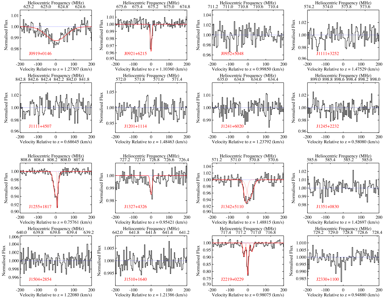
Figure 2. H I 21-cm absorption spectra towards the sample of strong Fe II systems, smoothed to \sim 4 \text{ km s}^{-1} . In the case of H I 21-cm absorption detections, individual Gaussian components and the resultant fits to the absorption profiles are overplotted as dotted and continuous lines, respectively. The quasar name as given in Table 1 is provided for each spectrum.
