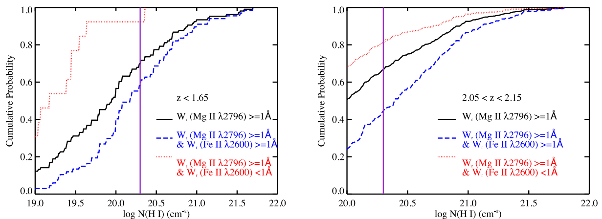
Figure 1. The cumulative distribution of \log N(\text{H I}) in systems with W_{\text{Mg II}} \geq 1 \text{ \AA} (solid), those with both W_{\text{Mg II}} \geq 1 \text{ \AA} and W_{\text{Fe II}} \geq 1 \text{ \AA} (dashed), and those with W_{\text{Mg II}} \geq 1 \text{ \AA} and W_{\text{Fe II}} < 1 \text{ \AA} (dotted). The left-hand panel shows the distribution for systems at z < 1.65 with N(\text{H I}) measurements from R06 using HST . The right-hand panel shows the distribution for systems at 2.05 < z < 2.15 from Zhu & Ménard (2013) with N(\text{H I}) measurements from Noterdaeme et al. (2012) using SDSS. The vertical line in each panel marks N(\text{H I}) = 2 \times 10^{20} \text{ cm}^{-2} .
