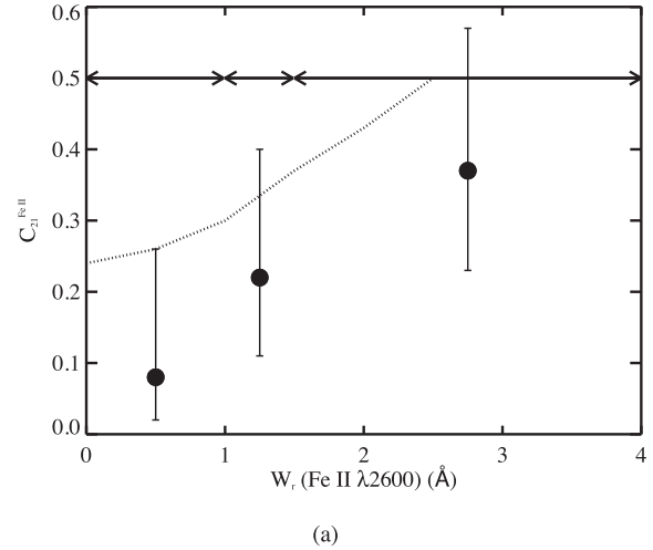
Figure 5. The detection rate of H I 21-cm absorption (for \tau_0 = 0.3 \text{ km s}^{-1} ) in three different bins (demarcated by arrows) of W_{\text{FeII}} for sample S2. The dotted line is the cumulative distribution of C_{21}^{\text{FeII}} , i.e. for W_{\text{FeII}} = x \text{ Å} , it gives C_{21}^{\text{FeII}} in systems with W_{\text{FeII}} \geq x \text{ Å} . The C_{21}^{\text{FeII}} estimate at W_{\text{FeII}} < 1 \text{ Å} are using measurements from G09 and G12.
