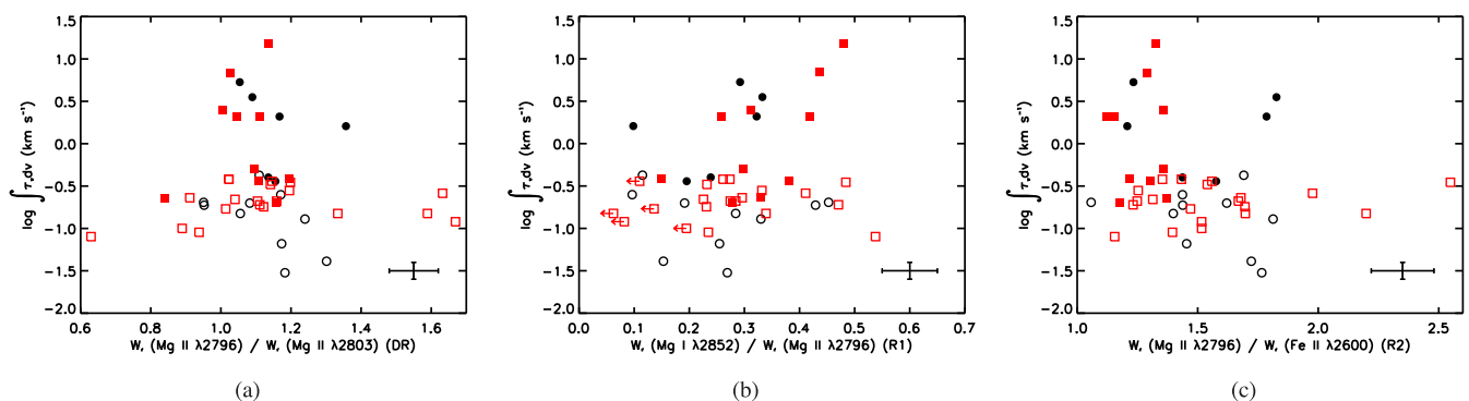
Figure 6. H I 21-cm absorption strength of the strong Fe II systems as a function of different metal line equivalent width ratios: (a) DR, (b) R1 and (c) R2. Black circles are for the systems in our sample and red squares are for the systems from G09 and G12. The filled symbols correspond to \int \tau dv of the H I 21-cm detections and the open symbols correspond to \int \tau dv_{10}^{3\sigma} of the non-detections. The typical error bars are plotted in the bottom right corner of each plot.
