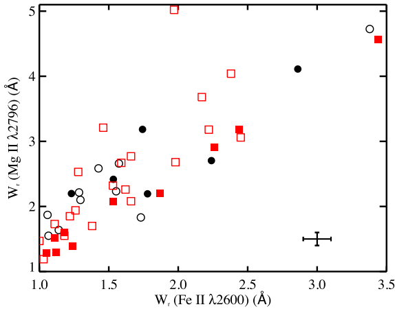
Figure 3. W_{\text{MgII}} versus W_{\text{FeII}} for the strong Fe II absorbers in our sample are shown as black circles and in the systems from G09 and G12 are shown as red squares. The filled symbols correspond to H I 21-cm detections and the open symbols correspond to non-detections. The typical error bars are plotted in the bottom right corner.
