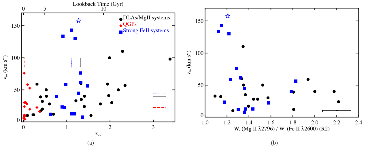
Figure 10. (a) The velocity width, v_{90} , of H I 21-cm absorption lines detected in samples of DLAs/Mg II systems (black circles), QGPs (red diamonds) and strong Fe II systems (blue squares). The solid, dashed and dotted vertical (horizontal) ticks mark the median z_{\text{abs}} ( v_{90} ) for the DLAs/Mg II systems, QGPs and Fe II systems, respectively. The measurement towards J0919+0146 from our sample (which is not considered in the analysis; see text for details) is shown as a star. (b) v_{90} of H I 21-cm absorption lines detected at 0.3 < z < 2.3 as a function of the ratio R2. The symbol convention is same as in panel (a). The typical error bar in R2 is plotted in the bottom right corner.
