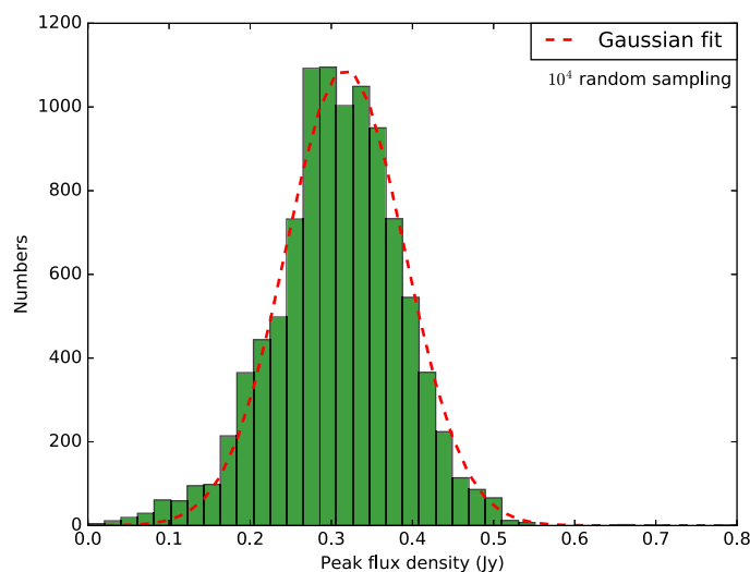
Figure C2. Distribution of the measured line fluxes, for a 10 000 times randomly sampled signal of 0.3 Jy Sinc function after baseline subtraction.
