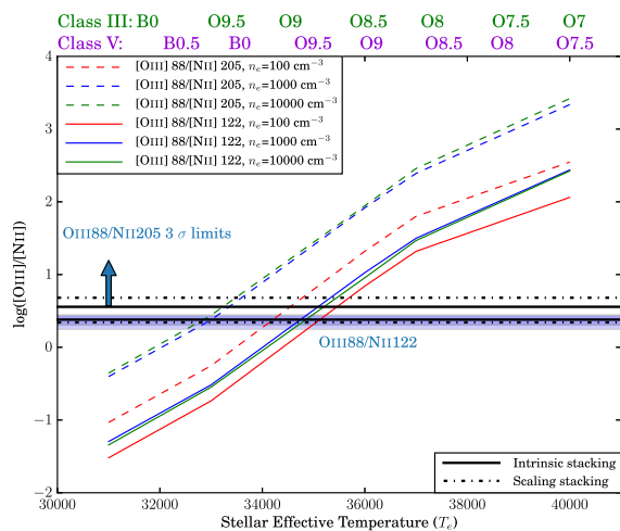
Figure 15. Theoretical line luminosity (in L_{\odot} ) ratio of [O III] 88 \mu\text{m} and the [N II] 122 \mu\text{m} lines as a function of the effective stellar temperature, derived from the Rubin (1985) H II models. We plot the observed [O III] 88 \mu\text{m} to [N II] 122 \mu\text{m} ratios and the upper limits of the observed [O III] 88 \mu\text{m} to [N II] 205 \mu\text{m} ratios, derived from for intrinsic stacking (black thick line) and scaling stacking (dash-dotted line), respectively. The upper axis labels show stellar types of OB stars of corresponding electron temperature for luminosity class III (Green) and luminosity class V (Purple) stars, according to the classification of Vacca et al. (1996).
