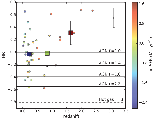
Figure 5. HR versus redshift and SFR (colour bar) for the 40 dwarf galaxies (filled dots). The dashed line indicates the HR of thermal emission with \Gamma = 3 , the solid lines represent the HR of hard X-ray emission from moderately obscured AGN with photon index \Gamma = 1 and Galactic N_H = 2.6 \times 10^{20} \text{ cm}^{-2} , and unobscured AGN with \Gamma = 1.4 , \Gamma = 1.8 and \Gamma = 2.2 and Galactic N_H . The error bar on the top right corner denotes the mean error of the 40 sources. The big squares are the mean HR of the redshift bins: 0 < z < 0.6 , 0.6 \leq z < 1.0 , and 1.0 \leq z < 2.4 .
