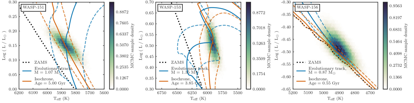
Fig. 8. WASP-151, WASP-153 and WASP-156 marginalized posterior distribution in the Hertzsprung–Russell diagram. The dotted black lines correspond to the zero-age main sequence (ZAMS) at best-fit [Fe/H]. This is defined as the time at which the star reaches its minimum luminosity and stellar ages are measured relative to this time. The blue lines are stellar mass evolutionary tracks and the orange ones are age isochrones. For both isochrones and evolutionary tracks the solid line correspond to the best-fit model (maximum of joint likelihood distribution) and the dashed lines correspond to the two extrema of the 68% confidence interval. For more details see Sect. 3.2.2 and Table A.6.
