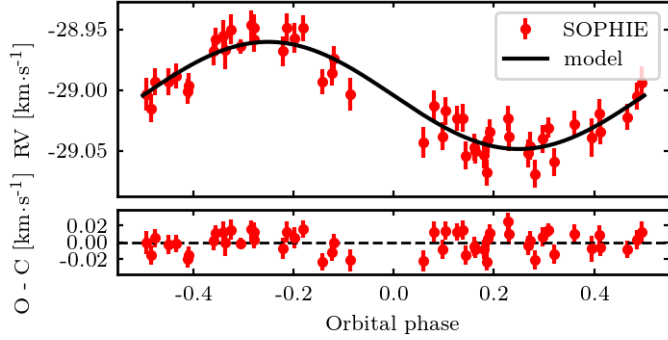
Fig. 5. Radial velocities of WASP-153. The data points are represented with their associated 1\sigma error bars.
