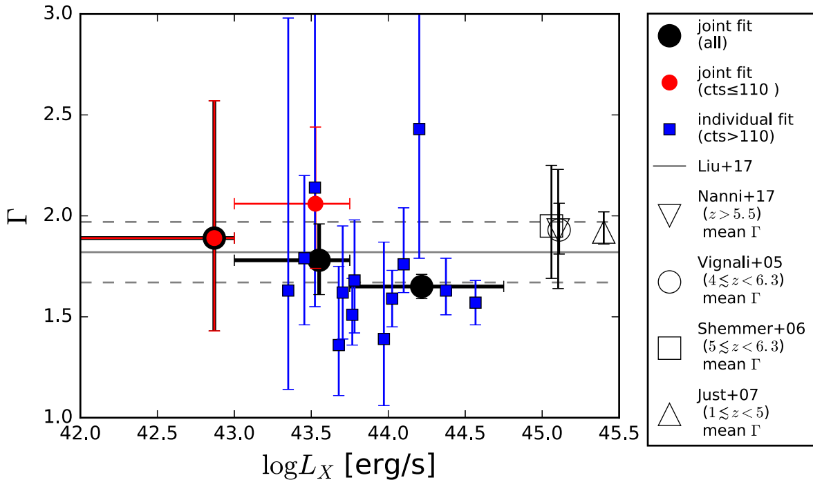
Figure B1. Best-fitting photon indexes for individual, bright sources with >110 net counts in the 0.5–7 keV band (blue squares), and the average values derived from a joint spectral analysis including all sources (black points) and only those with <110 net counts (red points), in three luminosity bins. No bright source lies in the first luminosity bin, where therefore the black and red points are coincident. Grey solid and dashed lines mark the median \Gamma derived by Liu et al. (2017) in the 7 Ms CDF-S and its standard deviation, respectively. We also show the average \Gamma of samples of luminous, optically selected Type-I QSOs in different redshift intervals.
