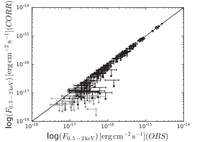
Figure 8. Best estimates of the soft-band flux obtained by integrating equation 16, with relative 68 per cent confidence level uncertainties, corrected for Eddington bias (see equation 5), compared to the uncorrected (i.e. observed) values. Grey symbols represent soft-band undetected sources, which are shown for completeness, for which the count rate (and therefore flux) in the hard band has been used everywhere else in this work.
