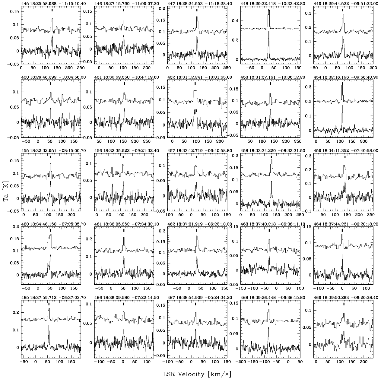
Fig. A.1. IRAM spectra of 86 GHz SiO maser lines. Each panel shows at the bottom the spectrum obtained with the autocorrelator ( 1.1 \text{ km s}^{-1} ), and at the top that obtained with the filter bank ( 3.5 \text{ km s}^{-1} , offset from zero). The line-of-sight velocity listed in Table D.1 is indicated with a small vertical bar at the top of each panel. The conversion factor between antenna temperatures and flux densities is 6.2 \text{ Jy K}^{-1} .
