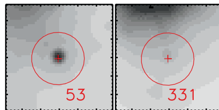
Fig. 4. MIPS GAL 24\mu\text{m} 1' \times 1' maps of the two targets located in Quadrant II of Fig. 3. Images have been bytescaled with a minimum at zero and a maximum at 500 MJy/sr (#53) or 1900 MJy/sr (#331). North is up and east to the left. The IRAM pointing positions are marked with circles of radius 14''.5 . The final retained 2MASS positions are marked with crosses.
