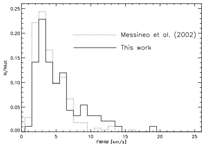
Fig. 2. Histogram of the SiO maser line widths. The solid line shows the distribution of the SiO masers presented in this work; the dotted line shows those previously published by Messineo et al. (2002). The numbers have been scaled to the total number (444) in the previous study and to the number 135 in the present study
