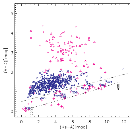
Fig. 5. 2MASS-MSX K_s-A versus A-D diagram of targets. SiO maser detections are marked with blue filled circles and non-detections with blue empty circles. Upper limits and blends have been removed. Identification numbers are as in Table D.2. The dotted line marks the separation between O-rich and C-rich shells found by Ortiz et al. (2005). The long-dashed line represents a blackbody ( F_{\nu} ) with temperature from 2200 to 400 K. New candidate C-type stars from our survey (see text) are labeled. For comparison K_s-A versus A-D values of the carbon stars analyzed by Ortiz et al. (2005) are overplotted with+++ magenta crosses, transitional objects with diamonds, and PNe with triangles.
