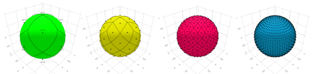
Figure 1: See how a sphere is first split into 12 base pixels of equal area whose centers are aligned at three different latitudes. Then, each is further subdivided to achieve higher and higher resolution.
