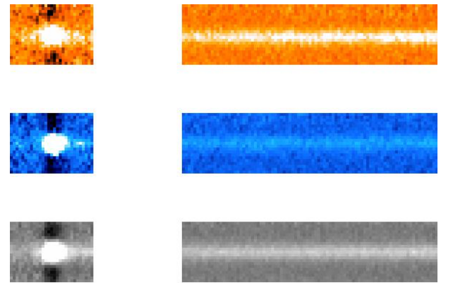
Fig. 13. Stacks of the 2D spectra of the LAEVs in the identified overdensities ( upper ), in the transition ( middle ), and field ( lower panel ) regions at the wavelength of Ly \alpha ( left panels ) and of the UV continuum at 1400 Å ( right panels ) rest frame.
