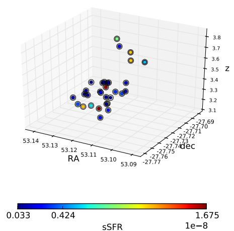
Fig. B.9. Same as Fig. B.1 for the overdensity detected at z = 3.29 in the CDFS.
