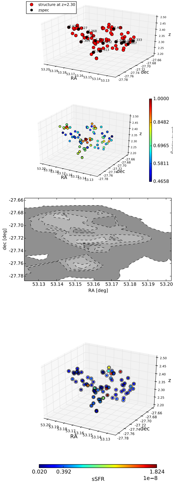
Fig. B.2. Same as Fig. B.1 for the overdensity detected at z = 2.30 in the CDFS.
