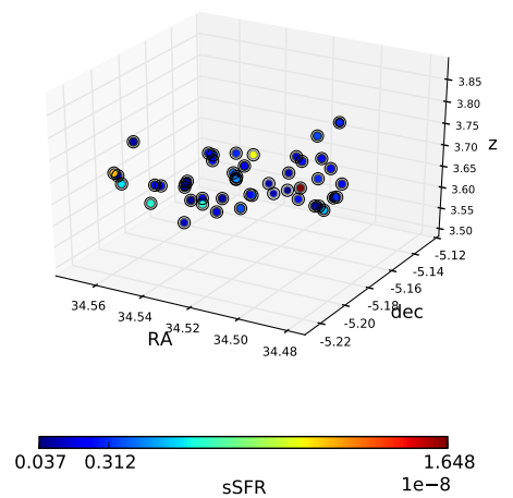
Fig. B.21. Same as Fig. B.1 for the overdensity detected at z = 3.69 in the UDS.
