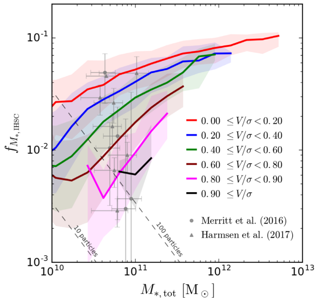
Figure 9. Same as Fig. 7, but the f_{M_*, \text{IHSC}} - M_* relation into subsamples of galaxies of different V/\sigma , as labelled. For clarity, we only show only 16th–84 th percentiles shaded regions. Observational estimates from Merritt et al. (2016) and Harmsen et al. (2017) are shown as grey symbols. It is clear that the f_{M_*, \text{IHSC}} does show an anticorrelation with the kinematic morphology V/\sigma of the central galaxy; the medians of each subsample do not overlap and show a continuous transition from high V/\sigma and low f_{M_*, \text{IHSC}} towards low V/\sigma and high f_{M_*, \text{IHSC}} . The observed behaviour is consistent with the expected active assembly history of galaxies supported mainly by dispersion, and a more quiescent one for rotationally supported ones. See the text for a more extensive discussion.
