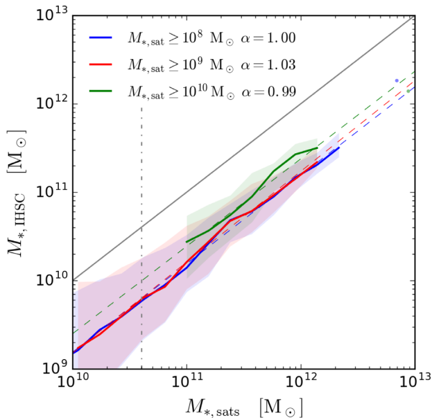
Figure 5. IHSC mass as a function of the total stellar mass in satellites with stellar masses >10^8 , 10^9 , and 10^{10} M_\odot , for f_{i,x,6D} = 0.4 . Solid lines shows the median in each mass bin, and shaded regions delimit the 16th and 84th percentiles. Similarly to Fig. 4 dashed lines show a power-law fit to the median. The mass relation between M_{*,\text{sats}} and M_{*,\text{IHSC}} is consistent even when only satellites with M_* > 10^8 and 10^9 M_\odot are used. For a mass threshold of 10^{10} M_\odot , the relation has a similar slope but is shifted towards the left.
