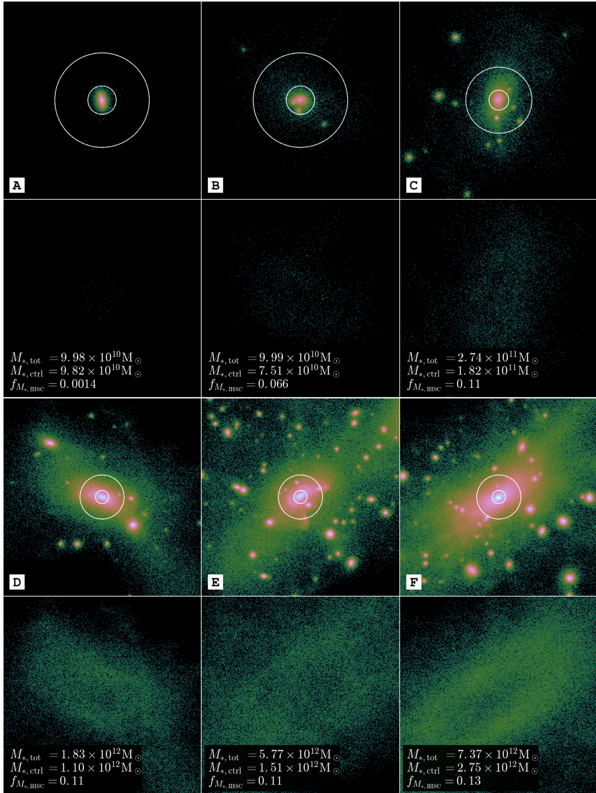
Figure 1. Projected stellar mass density of all the stellar particles inside 3DFOF objects (first and third rows), and its IHSC as identified using VELOCIRAPTOR (second and fourth rows). 3DFOF total stellar mass, M_{*, \text{tot}} , central galaxy stellar mass, M_{*, \text{ctrl}} , and IHSC mass fraction f_{M_{*, \text{IHSC}}} = M_{*, \text{IHSC}}/M_{*, \text{tot}} are shown for each object. Circles show 30 and 100 kpc apertures commonly used in the literature to separate the central galaxy from the stellar halo/ICL.
