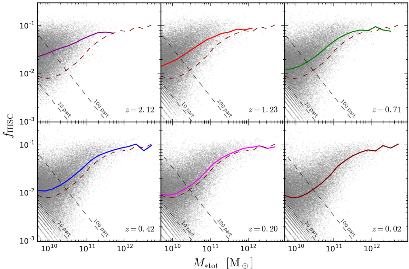
Figure 14. Temporal evolution of the f_{M_*,\text{IHSC}} - M_* relation from z = 2.12 to 0.02 , as labelled. Grey points are the measurements for individual systems; solid lines indicate the median f_{M_*,\text{IHSC}} per mass bin, and dashed line indicates the median at z = 0 for reference. Diagonal dashed lines indicate f_{M_*,\text{IHSC}} limits for IHSC composed 10 and 100 particles at a given M_{*,\text{tot}} , as labelled.
