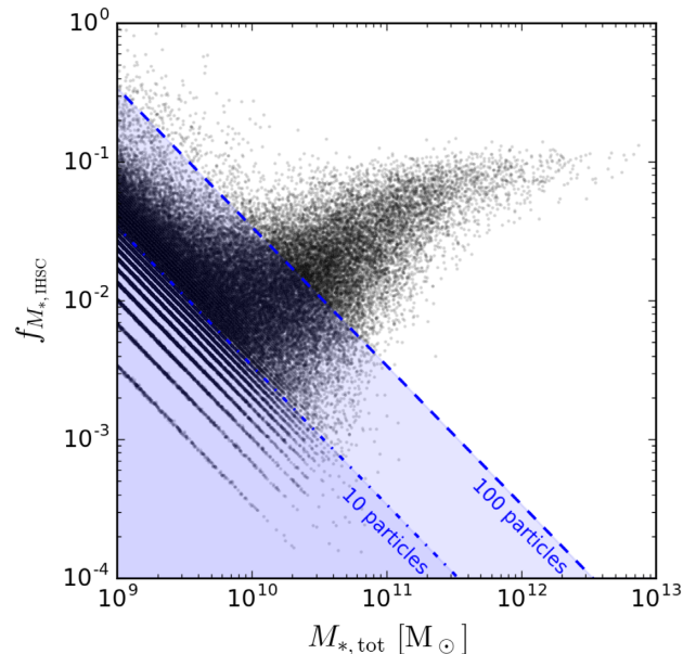
Figure 2. Mass fraction in the IHSC, f_{M_*,\text{IHSC}} , as identified by VELOCIRAPTOR, as a function of total stellar mass M_{*,\text{tot}} at z = 0 for all systems in the Horizon-AGN simulation, shown as black dots. Blue dashed and dotted-dashed lines delimit regions where the IHSC at a given M_{*,\text{tot}} is composed by \leq 100 and \leq 10 particles, respectively. See the text for more details.
