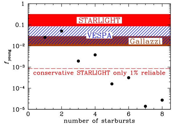
Figure 26. Comparison of prediction of mean fractions of very young galaxies of stellar mass m > 10^8 \text{ M}_{\odot} : predicted by the cosmic star formation history (from equation 11, filled circles ) and obtained from SDSS (from equation 12, shaded regions extending from conservative to liberal).
