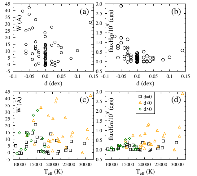
Fig. 11. Panel a: total equivalent widths in \text{\AA} of the H\alpha line emission components for Be stars against the sBD component d in dex. Panel b: fluxes of the H\alpha line emission components against the sBD d in dex. Panel c: total equivalent widths in \text{\AA} of the H\alpha line emission components against the apparent effective temperature. Panel d: fluxes of the H\alpha line emission components against the apparent effective temperature.
