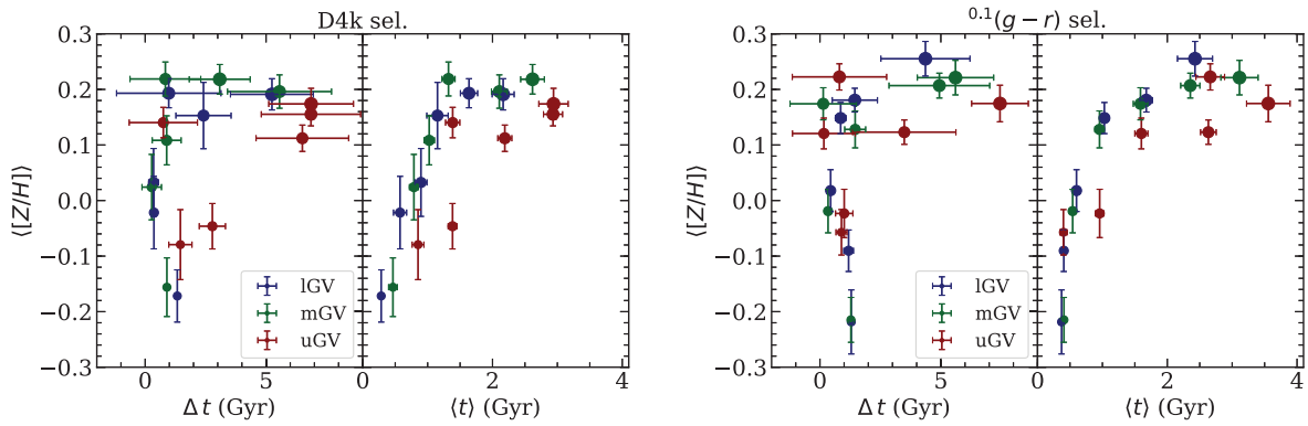
Figure 9. Trends between metallicity and either \Delta t or average age. The blue, green, and red data points show the results for IG, mGV, and uGV, respectively. The marker size follows velocity dispersion. The uncertainty in average metallicity remains constant, whereas the error bar in \Delta t_Q increases with average metallicity. Results are shown for the 4000 Å break selection (left) and the colour selection (right) of GV galaxies.
