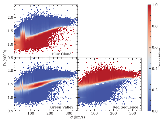
Figure D1. The probability of galaxies belonging to the BC (top left), Green Valley (bottom left), and Red Sequence (bottom right). Blue colours represent galaxies with a low probability of residing in the three regions, as labelled, while red shows high probability (see colour bar for reference). For ease of visualization, the resulting density plots have been modified with a Gaussian smoothing kernel.
