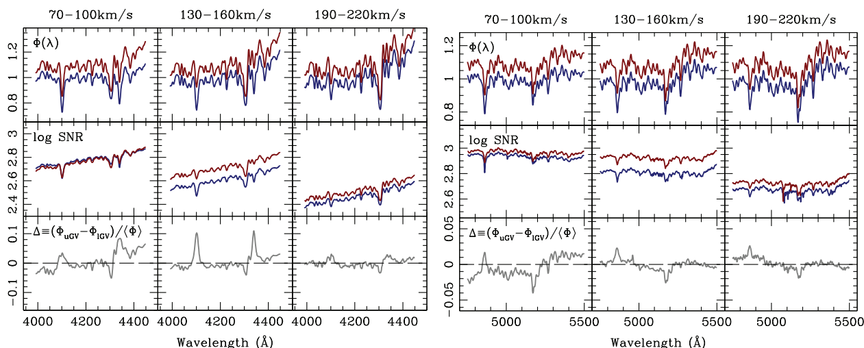
Figure 1. A comparison of the stacks is shown here in two important spectral windows: the neighbourhood of the H\gamma and H\delta absorption lines (left-hand panels) and the region around the H\beta and Mg+Fe complex (right-hand panels). From top to bottom, the panels show the fluxes of the IGv (in blue) and the uGV (in red), with a small arbitrary vertical offset to avoid crowding; the signal-to-noise ratio on a logarithmic scale; and the relative flux difference between uGV and IGv spectra. The top labels show the velocity dispersion in each case. All stacks have been convolved to a common velocity dispersion equivalent of 235 \text{ km s}^{-1} .
