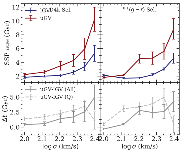
Figure 4. The SSP-equivalent age derived from line strengths is shown with respect to velocity dispersion in the IGV (blue) and uGV (red) subsets for the D4k- (left) and the colour-selected (right) GV. The bottom panels show the age difference between uGV and IGV stacks. These are derived from the stacks presented in this paper that comprise quiescent, star-forming, and LINER AGN galaxies. The dashed grey lines in the bottom panels contrast the results with A19, where the stacks only involve quiescent GV galaxies.
