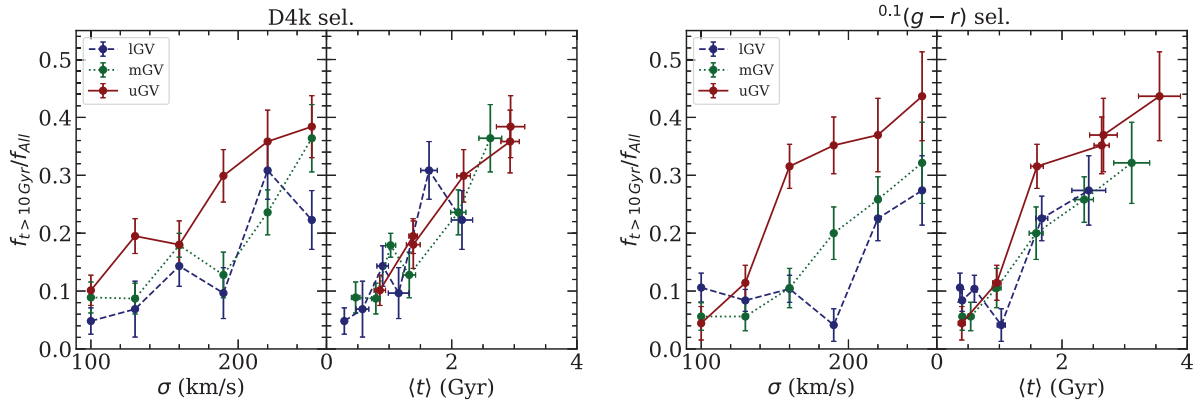
Figure 11. Relation between the mass fraction in old stellar populations ( \gtrsim 10 \text{ Gyr} ), with respect to velocity dispersion (left) and average age (right). The blue, green, and red lines correspond to IGV, mGV, and uGV galaxies, respectively. Results are shown for the 4000 \text{ \AA} break selection (left) and the colour selection (right) of GV galaxies.
