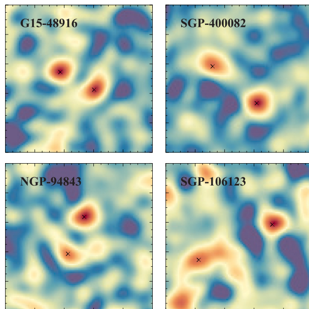
Figure 13. 76 \times 76 arcsec 2 AzTEC 1.1 mm SNR maps of the four most likely physically interacting galaxy candidates in the sample. All the detected sources fall within 36.6 arcsec of the original Herschel position (the beamsize at 500 \mu\text{m} ) and have individual photometric redshifts in agreement with each other within the error bars. These sources, which are typically missed in interferometric observations due to their small fields of view, are likely galaxy over-densities and/or pre-coalescence galaxy mergers.
