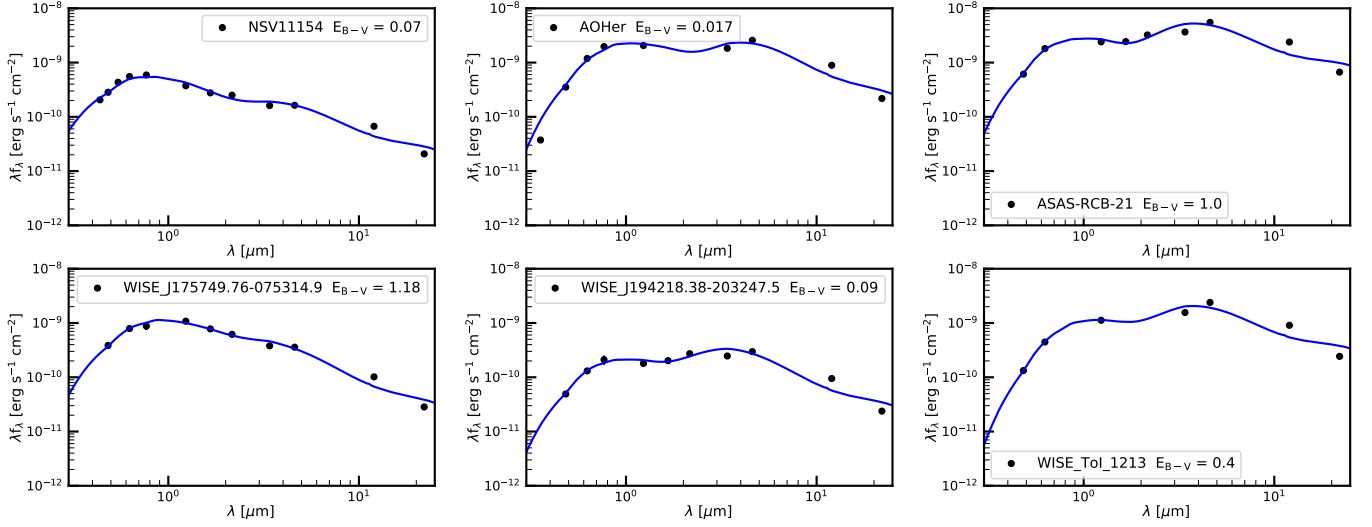
Figure 8. Maximum light spectral energy distributions (SEDs) for six RCB stars from our sample. We plot the best-fit DUSTY models in blue. For each star, we also indicate the assumed values of E_{B-V} . The derived model parameters are listed in Table 3
