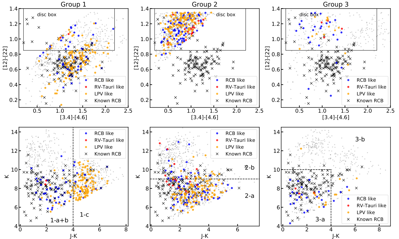
Figure 2. The WISE [3.4]-[4.6] vs [12]-[22] and 2MASS K vs J-K color-color diagrams for all candidates in the Tisserand et al. (2020) catalog. The left column shows the plots for candidates in Group 1, middle column shows candidates in Group 2 and the right column shows candidates in Groups 3. All candidates in each group are plotted as gray background points. On each color-color diagram, we highlight candidates that have light curves similar to RCB stars (Priority A, blue circles), RV Tauri stars (Priority E, red circles) and LPVs (Priority F, orange circles) present in the respective group. In addition, we also plot all known RCB stars as black crosses. We assign a new color based priority to each candidate based on its position in the K vs J-K diagram, as indicated. In the WISE color-color plots, we also indicate the “disc-box” where RV-Tauri stars surrounded by dust discs are expected to lie ( Gezer et al. 2015 ). In Group 1, J-K = 4 line separates LPVs from the known RCB stars and lc-Priority A candidates. We assign all candidates in Group 1 that have J-K < 4 mag and lie outside the RV-Tauri disc box to “Group-1-a” and those inside the disc box to “Group-1-b”. For Groups 2 and 3, we cannot identify a similar distinction between LPVs and RCB candidates. Instead, we use the positions of known RCB stars and our light curve based priority A candidates to prioritise these groups for spectroscopic followup (see text). We prioritise candidates in Group-1-a, Group-2-a and Group-3-a for spectroscopic followup.
