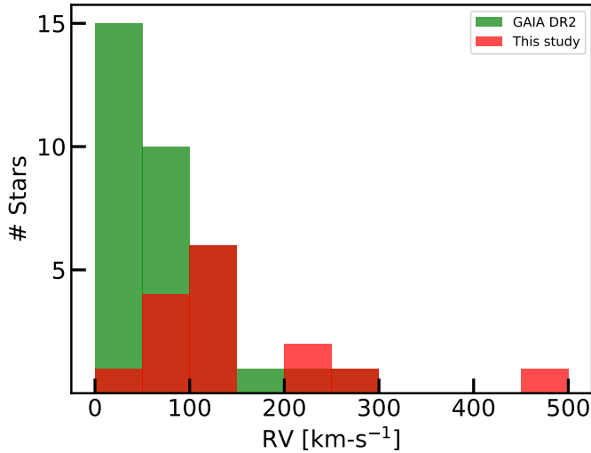
Figure 13. Distribution of the radial velocities of RCB stars. Previously known velocity measurements from GAIA DR2 are plotted in green and measurements from this study are plotted in red. We note that two RCB stars have very high radial velocities ( \approx 300 km/s), which could be indicative of a halo population for these objects.
