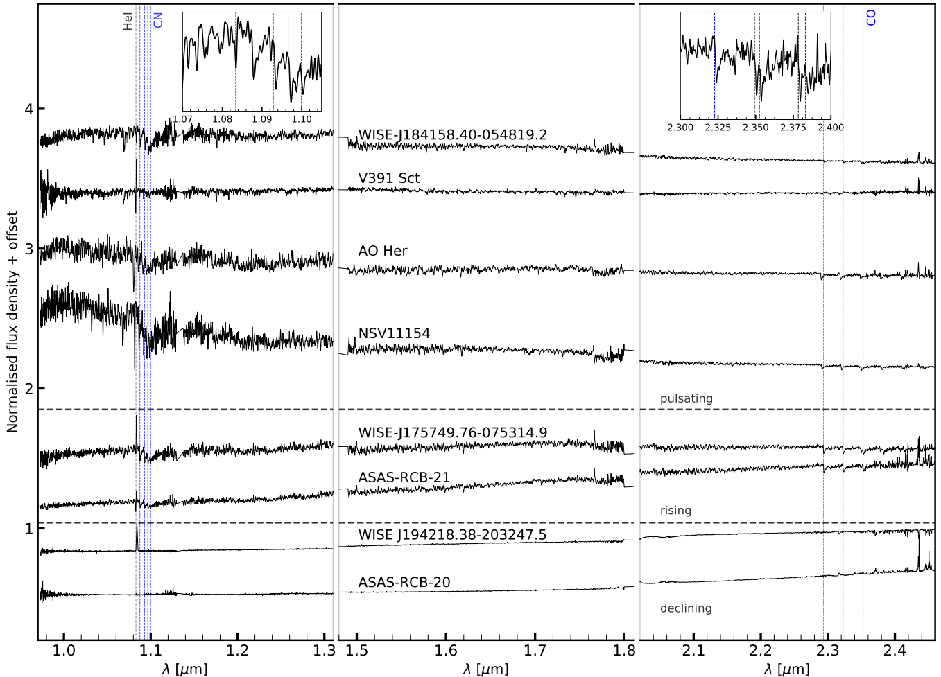
Figure 5. NIR spectra of 8 known RCB stars on 2019 November 23. The stars are grouped by their photometric phase - 4 pulsating, 2 rising and 2 fading. We also show a zoom in of the J-band and K-band spectra of the RCB star WISE-J18+. In the J-band inset plot, we mark the positions of the CN absorption bandhead in blue and He I absorption in gray. In the K-band inset, we mark the position of ^{12}\text{C}^{16}\text{O} and ^{12}\text{C}^{18}\text{O} absorption bandheads in blue and black respectively.
