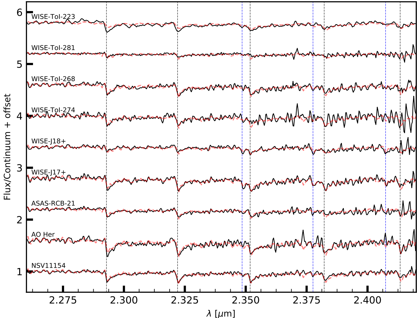
Figure 9. Best-fits to the K band spectra of RCB stars. The continuum normalised spectra are plotted as black solid lines and the best-fit synthetic spectra are plotted as red dashed lines. We mark the positions of ^{12}\text{C}^{16}\text{O} (black lines) and ^{12}\text{C}^{18}\text{O} (blue lines) absorption bandheads. The derived ranges of best-fit temperatures and oxygen isotope ratios are listed in Table 3.
