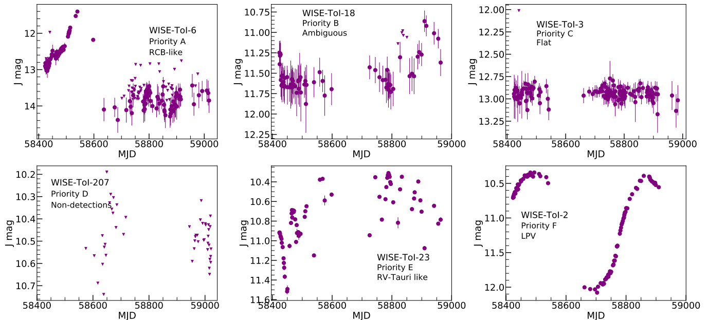
Figure 1. Examples of PGIR J-band lightcurves for candidates in each of the lc-based priority groups described in Section 2. The solid dots represent detections and triangles represent 5\text{-}\sigma upper limits. Of the 1209 candidates from Tisserand et al. (2020) catalog that have PGIR coverage, we assign 149 candidates Priority A (RCB-like), 279 candidates Priority B (ambiguous light curves), 199 candidates Priority C (flat light curves), 287 candidates Priority D (no detections), 23 candidates Priority E (RV Tauri-like) and 272 candidates Priority F (LPV-like). The Priority A group is expected to be rich in RCB stars, but the groups B, C and D could also contain RCB stars.
