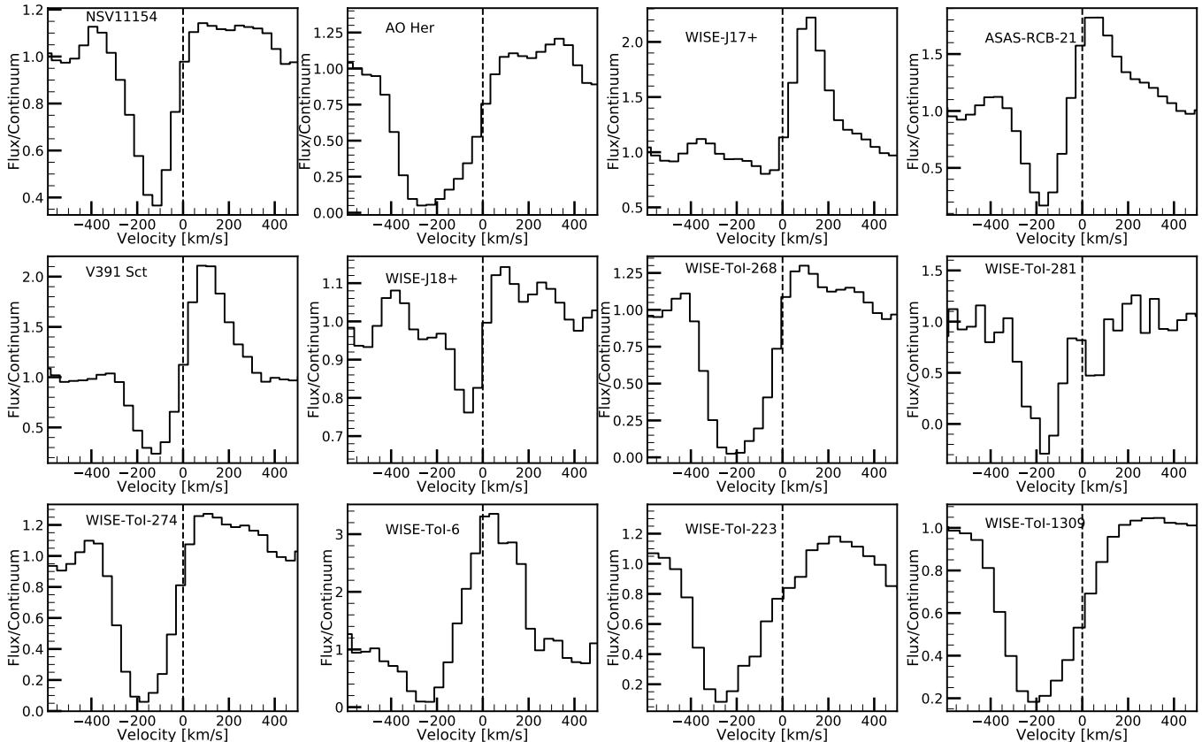
Figure 12. He I \lambda 10830 line profiles of RCB stars analysed in this paper. The helium line is an almost ubiquitous feature of RCB stars. This line originates in high velocity winds in the atmospheres of these stars. Some RCB stars show a fully developed p-cygni profile, while some stars show only the blueshifted component. In the latter case, other photospheric absorption reduces the emission component. Here, we have excluded the 7 RCB stars that are in a dust enshrouded dip, as we cannot derive radial velocities for them. These stars show the helium line in emission. The absorption component is absent as almost all the continuum is extinguished due to dust.
