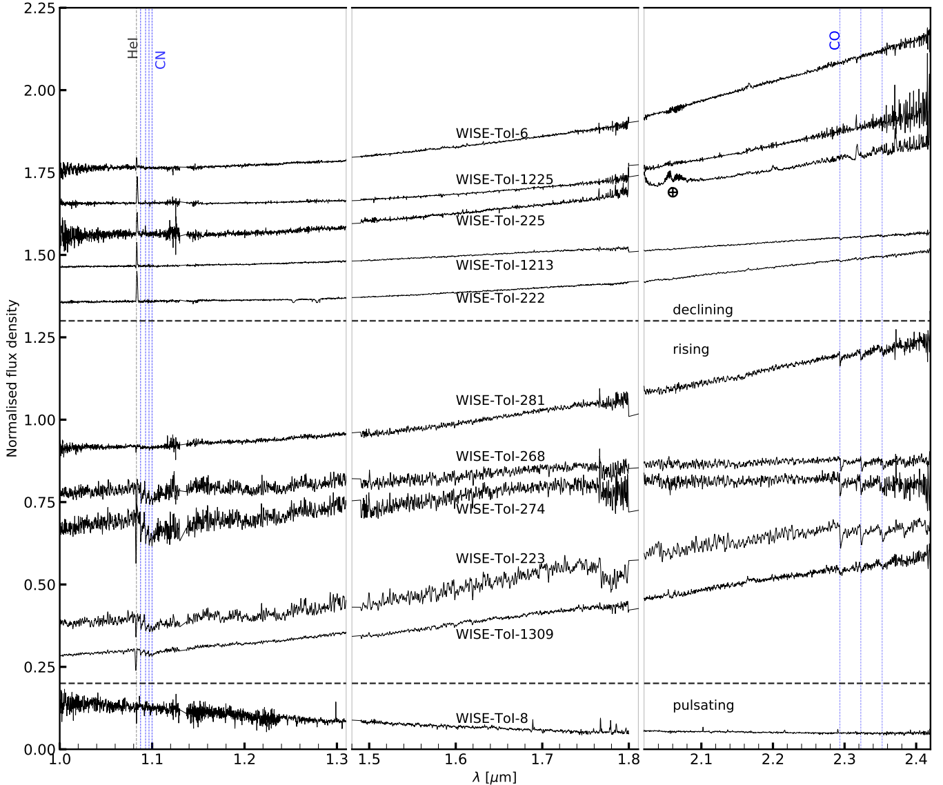
Figure 7. NIR spectra of new RCB stars identified in this paper. All RCB stars show He I \lambda 10830 features. 5 RCB stars that were in a deep decline show strong emission, while others show either fully developed p-cygni profiles or strong blueshifted absorption. 4 RCB stars show the CO absorption bandhead, suggesting that they are cold.
