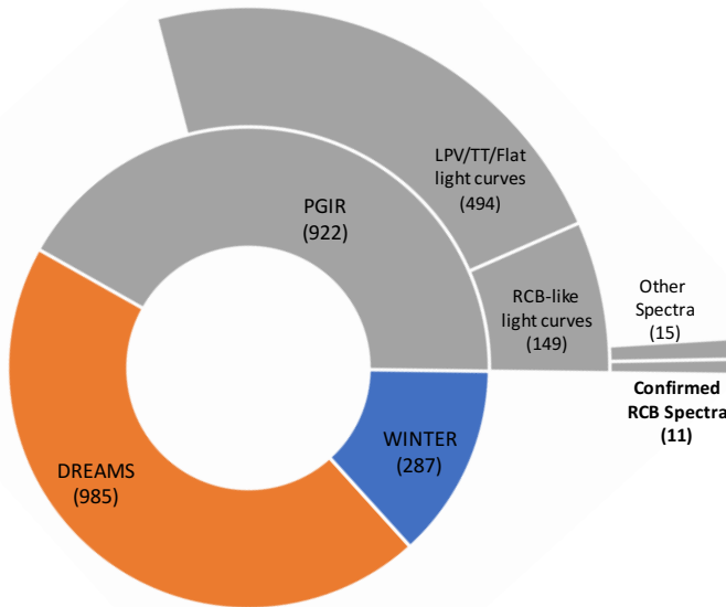
Figure 14. A schematic of our strategy for an NIR survey of Galactic RCB stars focusing on the Tisserand et al. (2020) catalog. 1209 candidates from this catalog are accessible from the northern hemisphere. Of these, 922 candidates are bright enough to be characterised by PGIR. The remaining 287 fainter candidates will be characterised by WINTER – a deeper ( J \approx 20 ) NIR time domain survey starting December 2021. The candidates in the southern hemisphere will be characterised by DREAMS, an analog of WINTER in Australia.
