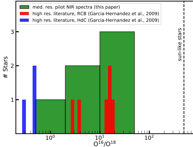
Figure 10. Distribution of ^{16}\text{O}/^{18}\text{O} ratios of RCB and HdC stars. In red, we plot all 6 previously available measurements of the isotope ratios in RCB stars derived from high resolution spectra García-Hernández et al. (2009) . In this paper, we report preliminary constraints on ^{16}\text{O}/^{18}\text{O} for 4 new RCB stars. We indicate these new measurements in green. We note that 5 additional RCB stars reported in this paper show weak ^{12}\text{C}^{18}\text{O} absorption features, and are consistent with ^{16}\text{O}/^{18}\text{O} > 10 . In blue, we plot the isotope ratios measured for HdC stars, taken from García-Hernández et al. (2009) . The high ^{18}\text{O} content of RCB stars compared to sun-like stars favours a white dwarf merger origin for them. Further NIR spectroscopic observations that populate this diagram will provide additional clues about the formation channels of RCB stars.
