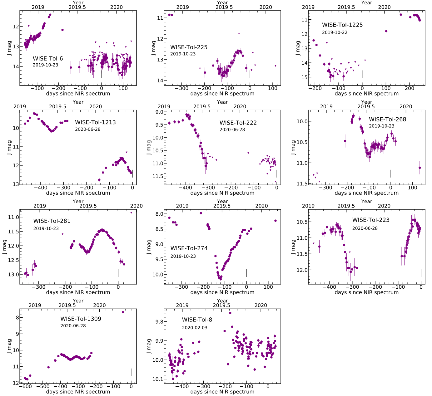
Figure 6. PGIR J band light curves of new RCB stars identified in this paper. The black vertical lines at 0 days mark the epochs at which the NIR spectra were acquired. For each RCB star, we also indicate the date when the spectrum was obtained. We note that photometry brighter than 8.5 mag may not be reliable due to non-linearity effects in the detector. All J-band magnitudes are in Vega system.
