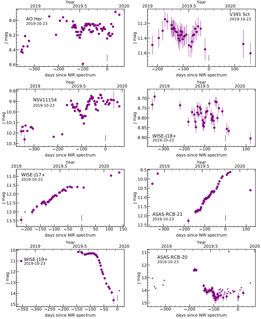
Figure 4. PGIR J Band light curves for 8 known RCB stars. The black vertical lines at 0 days mark the epoch at which the NIR spectra were acquired (indicated in each plot). We note that photometry brighter than 8.5 mag may not be reliable due to non-linearity effects in the detector. The J -band magnitudes are in Vega system.
