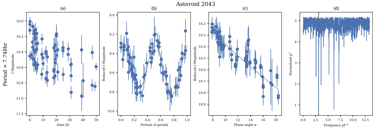
Figure 2. Lightcurve and analysis results output for Asteroid 2043 Ortutay. (a) shows the observed lightcurve with the distance correction applied. The zero date was set at the time of the first observation. Further figures may have observations in additional colours based on temporal grouping. (b) shows the folded lightcurve at the best-fitting period, with distance and phase effects removed. The calculated lightcurve model is shown in grey. (c) shows the observed phase relationship with the rotational model subtracted. The fitted phase model is shown in grey. (d) shows the periodogram at the best-fitted phase parameter. The black dotted line indicates the best-fitted frequency and the grey lines around it indicate the 1\sigma uncertainty frequency bounds.
