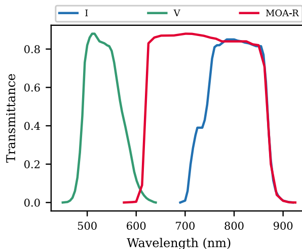
Figure 1. The MOA-II colour filters compare to standard Cousins filters. The MOA-R filter is used for the majority of Galactic Bulge observations and has a similar response to I band filters (Bond et al. 2001). V band observations are occasionally taken by the survey but were not used in this work.
