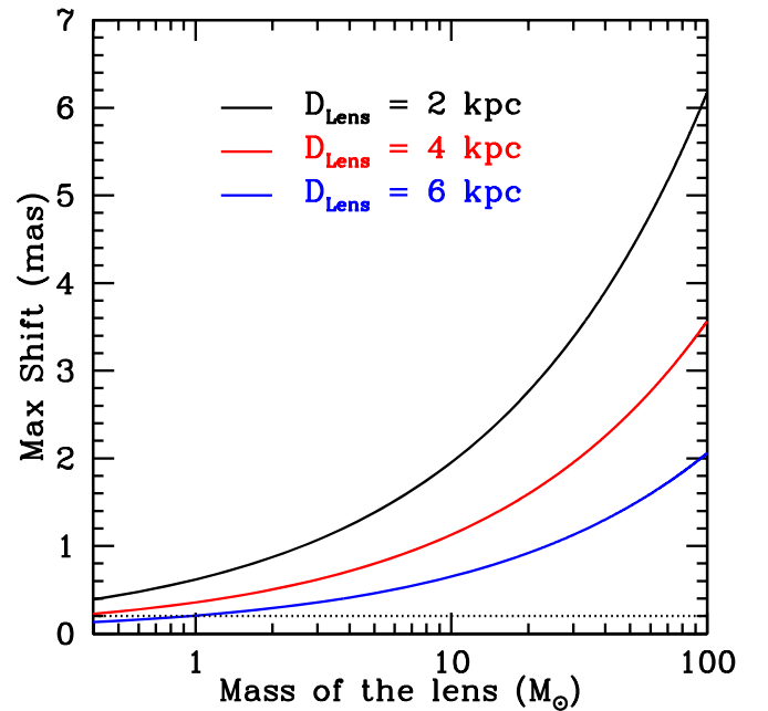
Figure 3. Maximum astrometric shift of a source in the Galactic bulge at 8 kpc as a function of lens mass, for lens distances of 2, 4, and 6 kpc. Since the maximum astrometric shift occurs at a lens–source separation of u = \sqrt{2} , while the maximum light magnification occurs at the minimum value of u , all high-magnification microlensing events will pass through the point of maximum astrometric deflection. High-S/N imaging with HST allows measurements of astrometric shifts with a precision of \sim 0.2 mas per observation epoch, shown by the dotted line at the bottom.
