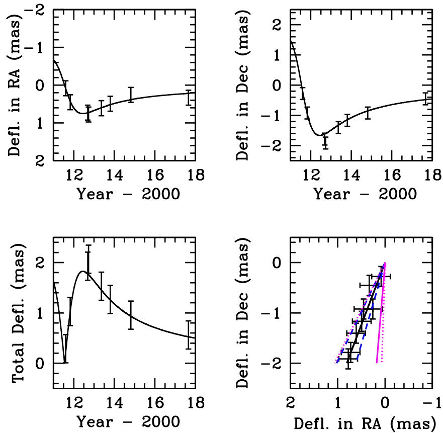
Figure 16. The top two panels show the average values of the measured deflections in R.A. and decl. at each HST epoch. We use the values of t_0 , t_E , and u_0 as derived from a light-curve fit without parallax, and fit for the proper motion of the source, \theta_E , and \varphi_{LS} . The solid black line is the best fit with \theta_E = 5.2 mas and \varphi_{LS} = 337^\circ.9 . The bottom left panel shows the total deflections at each epoch. The bottom right panel shows the R.A. vs. decl. deflections. These deflections are always along the line joining the lens to the source, and thus at large separations their direction is opposite to the direction of the relative motion of the lens with respect to the source. The solid black line passes through the origin, at the \varphi_{LS} angle derived above. The dotted blue lines indicate the allowed range from astrometry based on the uncertainties. The allowed range of \varphi_{LS} from photometry alone is shown by the dotted magenta lines, the best-fit value being \varphi_{LS} = 354^\circ.8 shown by the solid magenta line. The combined constraint from photometry and astrometry is used in our subsequent analysis.
