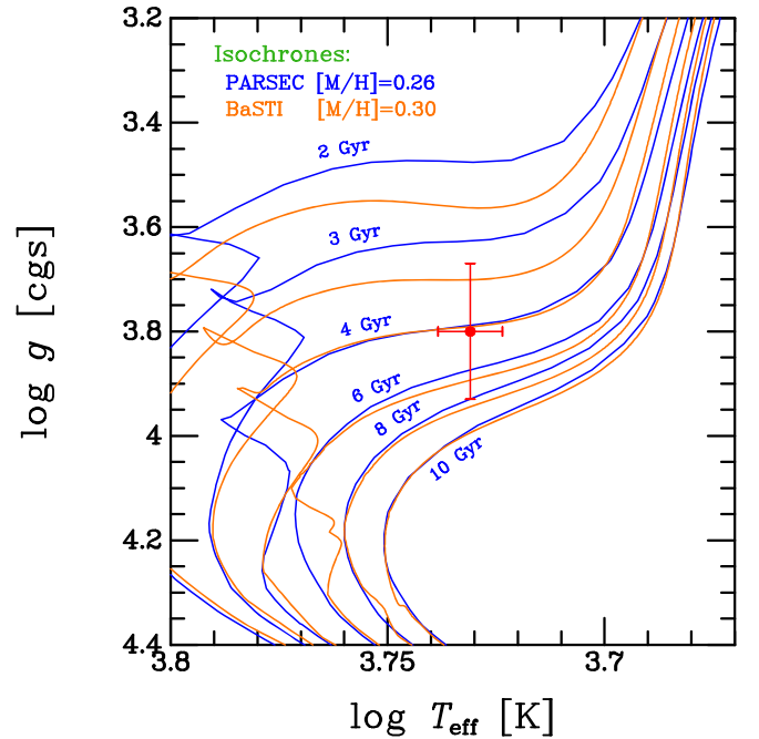
Figure 19. Location of the MOA-11-191/OGLE-11-462 source star in the \log g vs. effective temperature diagram (red filled circle with error bars), using stellar parameters from Bensby et al. (2013). Superposed are theoretical stellar isochrones from two sources. The blue curves show PARSEC isochrones, calculated for the source’s measured metallicity of [\text{M}/\text{H}] = +0.26 , for ages of 2–10 Gyr. The orange curves are BaSTI isochrones for [\text{M}/\text{H}] = +0.3 and the same range of ages.
