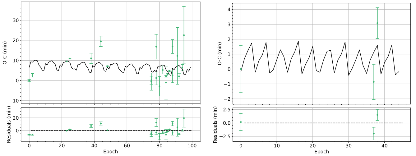
Figure 4. Two-planet O - C diagram of AU Mic b (left) and AU Mic c (right), with comparison between TTVs (green) and Exo-Striker-generated best-fit models (black).
