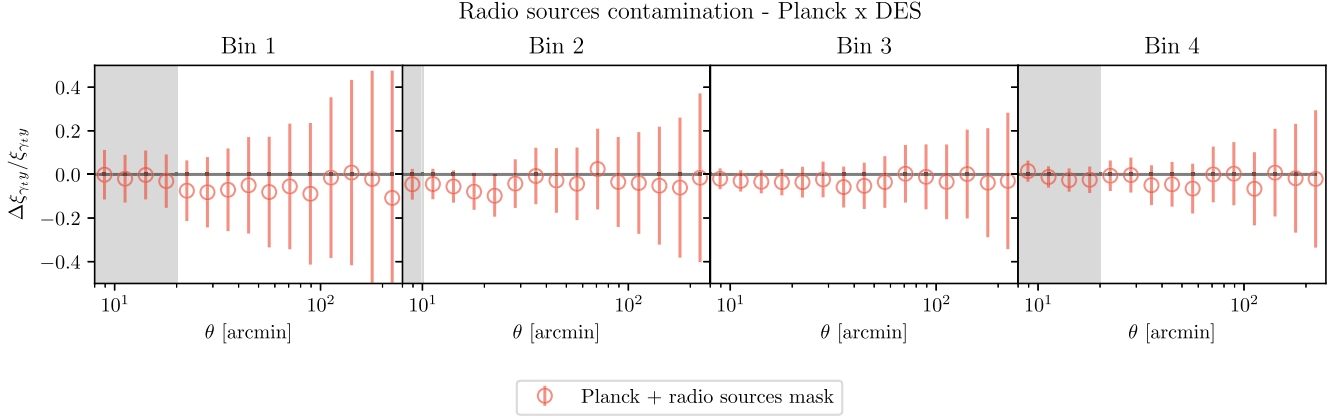
FIG. 7. Fractional difference in the measured shear-Compton- y cross-correlation \xi^{\tau,y} when computed using the Planck Compton- y map with and without masking radio sources. No statistically significant difference is measured, indicating no contamination due to radio sources. Gray shaded regions represent the scales removed in the main analysis.
