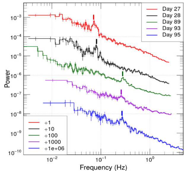
Figure 1. Optical QPOs from SHOC and SALT LS power spectra, identified with colour coding for each day (see the box) and arbitrary offsets with power. The vertical bars mark the value of the NICER X-ray QPO fundamental frequencies (Stiele & Kong 2020), apart from those on days 93 and 95, which are inferred from the upper harmonic values.
