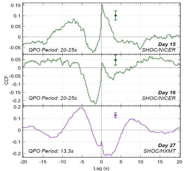
Figure 4. Optical/X-ray CCFs for the SAAO-SHOC versus NICER data obtained on days 15 (top panel) and 16 (middle panel) (dark green), and SAAO-SHOC versus Insight -HXMT on day 27 (bottom panel, dark violet). Each CCF is made from the average of 30-s segments, with a representative standard error bar shown. Note the precognition dip present in days 15 and 16, which evolves into a broad anticorrelation by day 27. Also note the sub-second peak at positive lags, which changes in shape over time.
