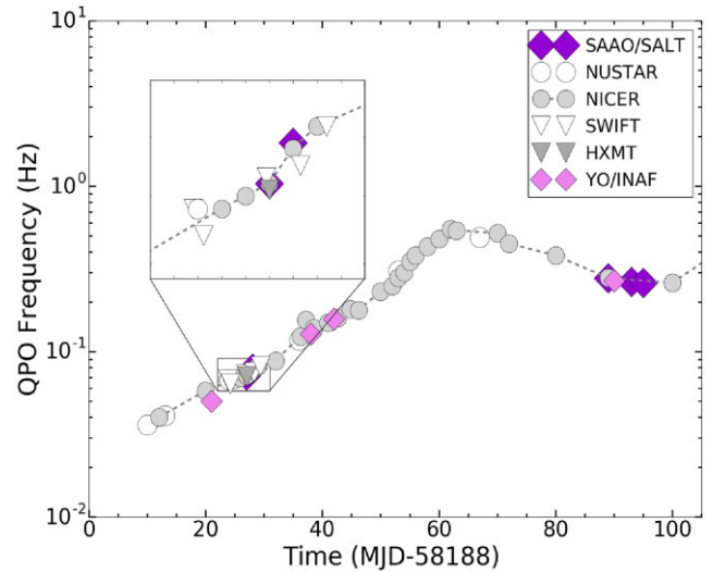
Figure 3. Temporal evolution of the optical and X-ray QPOs detected through the hard state of the J1820 outburst. The grey dotted line represents a polynomial fit to the Stiele & Kong (2020) NICER QPO fundamental frequencies. See the box (and text) for observatory identifications.
