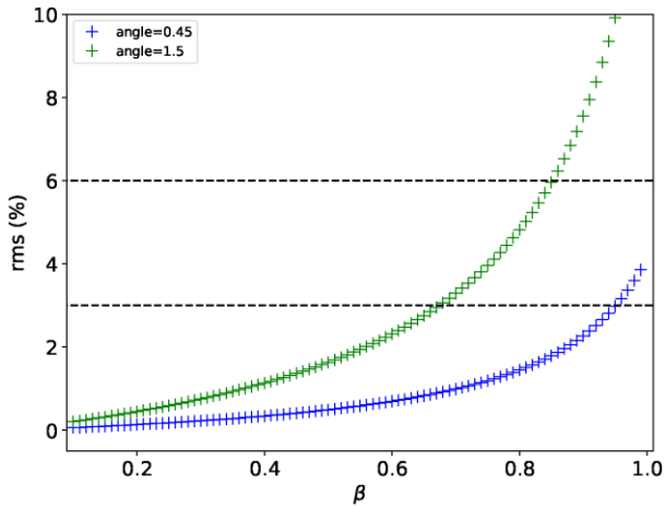
Figure 5. Relation between QPO rms and \beta ( =v_{\text{jet}}/c ) for opening angles of \phi = 1.5^\circ (green; Zdziarski et al. 2021b) and 0.45^\circ (blue; Tetarenko et al. 2021). The lower horizontal dashed line indicates the original QPO rms of 3 per cent, while the upper line indicates the QPO rms of 6 per cent from the jet when considering the contribution of the disc emission to the optical flux (Shidatsu et al. 2018).
